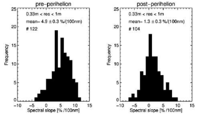
Fig. 7. Histograms showing the bright spots spectral slopes, evaluated in the 535–882 nm wavelength range, in images having similar high resolution (in the 0.33\text{--}1 \text{ m px}^{-1} range), in the pre-perihelion (August 2014–May 2015), and post-perihelion (November 2015–September 2016) periods.
