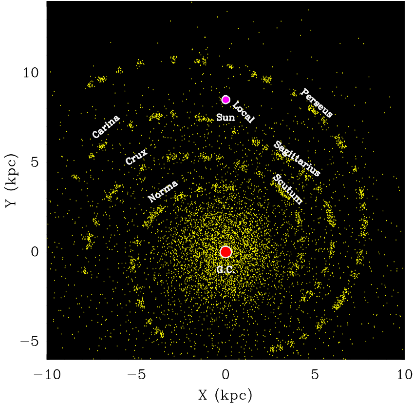
Figure 1: “Plan-view” model of the spiral structure of the Milky Way after Georgelin & Georgelin (1976) and Taylor & Cordes (1993). The main spiral arms are labeled. The red and purple dot indicate the position of the Galactic Center and the Sun, respectively.
