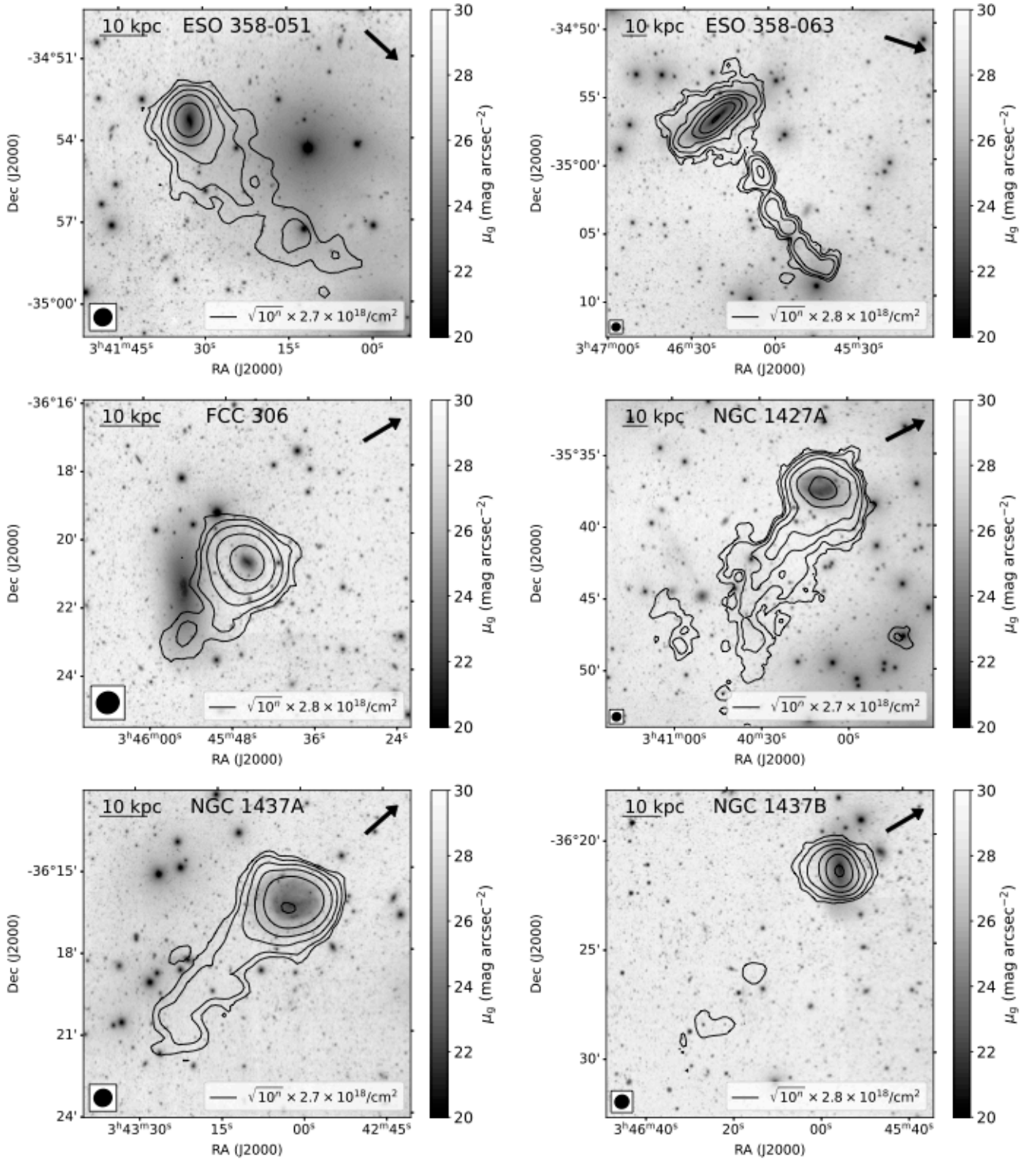
Fig. 9. MeerKAT H I contours overlaid on a g -band image from the Fornax Deep Survey for the six galaxies with a one-sided H I tail. The galaxy name is given at the top of each image. The H I contour levels are given in the bottom right legend ( n = 0, 1, \dots ). The bottom left black ellipse represents the 41'' H I resolution. The scale bar in the top left corner indicates 10 kpc. The top right arrow points towards NGC 1399 at the centre of Fornax.
