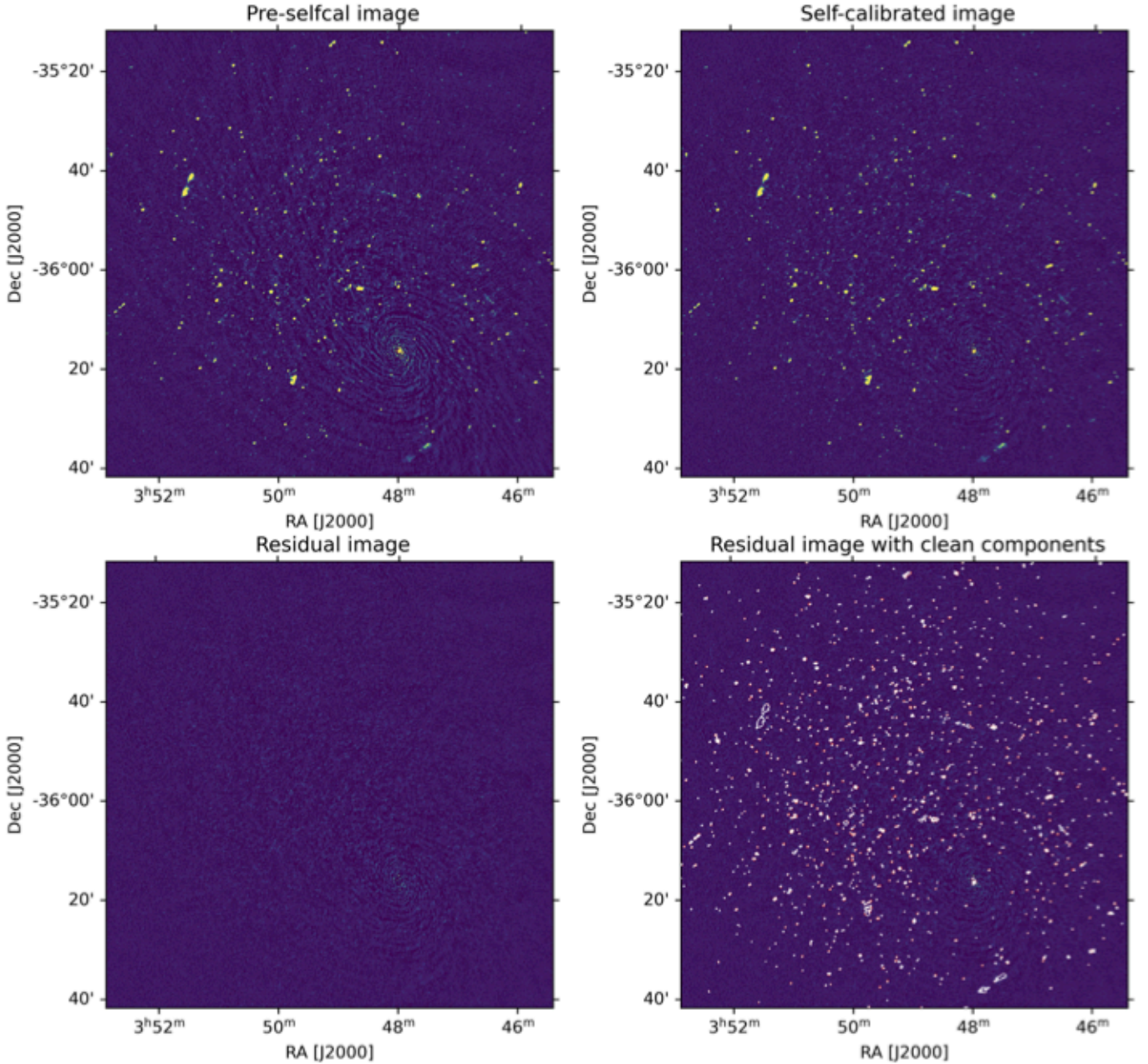
Fig. 4. Result of our imaging and self calibration loop for a typical MeerKAT 5-h observation. From left to right, top to bottom: the continuum image before self calibration; the continuum image after the last round of self calibration, showing the improved dynamic range; the last residual image, showing a population of faint sources not included in our sky model; and the residual image with white and red contours representing positive and negative clean components, respectively, demonstrating that our strategy minimises the inclusion of calibration artefacts around bright sources into the sky model. All images show a 2 \times zoom-in of the full imaged field and are on the same linear colour scale from -20 to +300 \mu\text{Jy beam}^{-1} (for comparison, the typical noise level is \sim 7\text{--}10 \mu\text{Jy beam}^{-1} ).
