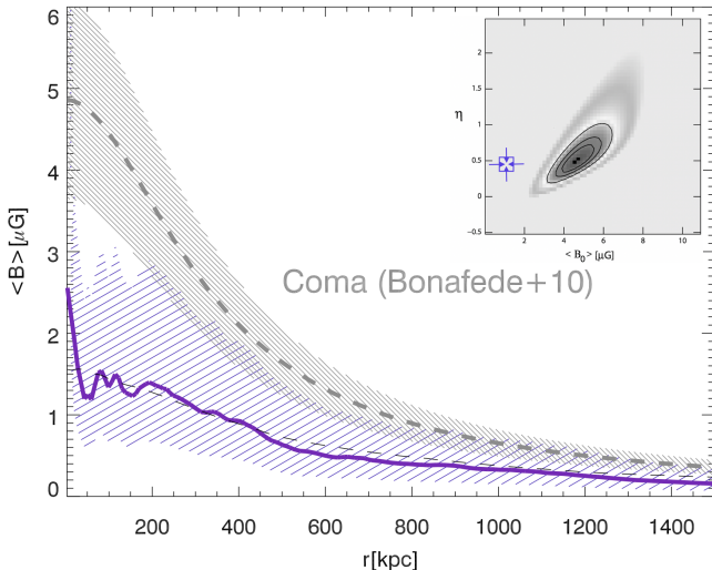
Figure 5. Radial profile of magnetic field in our most resolved run AMR8, compared to the magnetic field profile inferred by Bonafede et al. (2010) from observed RM. The dashed region of the profiles show the \pm 1\sigma dispersion around the mean. The dashed line shows the best fit to our measured profile, while the inset show the uncertainty region of the best-fit in Bonafede et al. (2010). The best fit solution for our the profile of our simulated cluster is shown by the purple cross.
