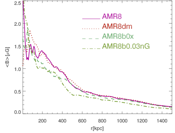
Figure 16. Radial profiles of the median magnetic fields at z = 0 for additional resimulations testing the role of the initial seed field (AMR8b0x and AMR8b0.03nG, see Tab. 1 for details) and of the mass resolution (AMR8dm).
