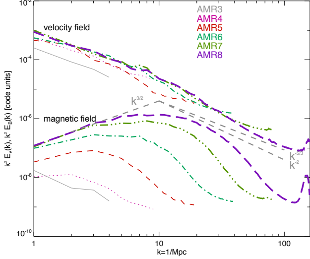
Figure 9. Spectral properties of the velocity and magnetic fields of our runs, as a function of resolution. The top lines show the velocity field power spectra (including also the weighting for n^{0.5} as explained in the text), while the bottom lines show the magnetic field power spectra for the innermost (1 Mpc) 3 volume of our cluster at z = 0 , for different spatial resolutions. The additional gray lines show the k^{3/2} and the k^{-5/3, -2} trends to guide the eye.
