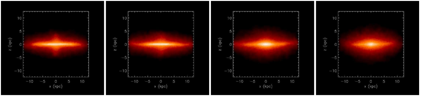
Figure 19. Edge-on view of gas density maps for different values of the Plummer-equivalent gravitational softening: \epsilon_{\text{Pl}} = 0.1, 0.3, 0.65, 1.3 \text{ kpc } h^{-1} (from left-hand to right-hand panels).
