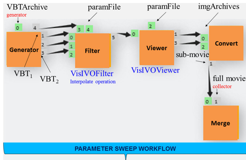
Figure 4. Dynamic Movie Workflow interpolates several steps of a time evolution of a cosmological dataset.
