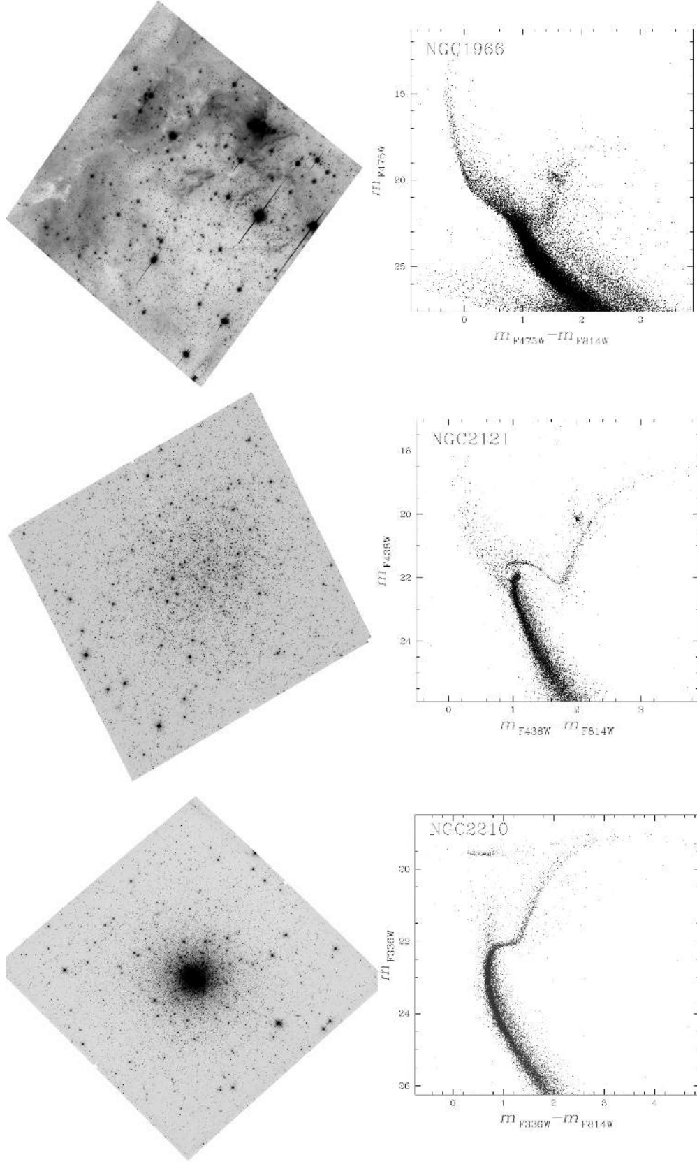
Fig. 4. Stacked images and CMDs of stellar fields with different ages and stellar densities. North is up and east to the right. Top panels: F475W image and the m_{F475W} vs. m_{F475W} - m_{F814W} CMD of stars in the star-forming region around the very young cluster NGC 1966. Middle and bottom panels: illustrate the F814W stacked images and the CMDs of the intermediate-age cluster NGC 2121 (age \sim 3 Gyr) and the old GC NGC 2210 (age \sim 12 Gyr), respectively.
