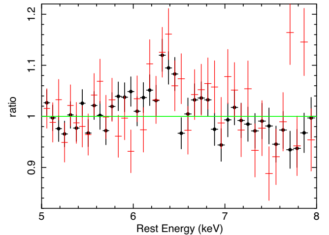
Figure 2. Suzaku XIS 0.3 data in the Fe K regime: 2010 (red) and 2007 (black) compared to a local power-law continuum model over 5–8 keV. A weak, but narrow, iron K \alpha emission line is seen near to 6.4 keV in the QSO rest frame.
