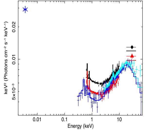
Figure 6. Unfolded data versus the best-fitting multiepoch OPTXAGNF model from Table 1: symbols as for Fig. 5. Note that for the Suzaku PIN data, the model is corrected for the calibration cross normalization factor (relative to XIS), but the data are not corrected.
