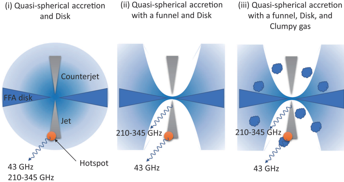
FIG. 3.— Schematic image of possible accretion flow structures. (i) 210-345 GHz emission is dominant in the hotspot. Faraday rotation is caused by RIAF. (ii) 210-345 GHz emission is dominant in the inner jet. Funnel zones are created by the previous jet activities, which causes a decrease of Faraday rotation as compared to the case (i). (iii) The jet is interacting with a clumpy gas, which responsible for the observed Faraday rotation toward the hotspot at 43 GHz.
