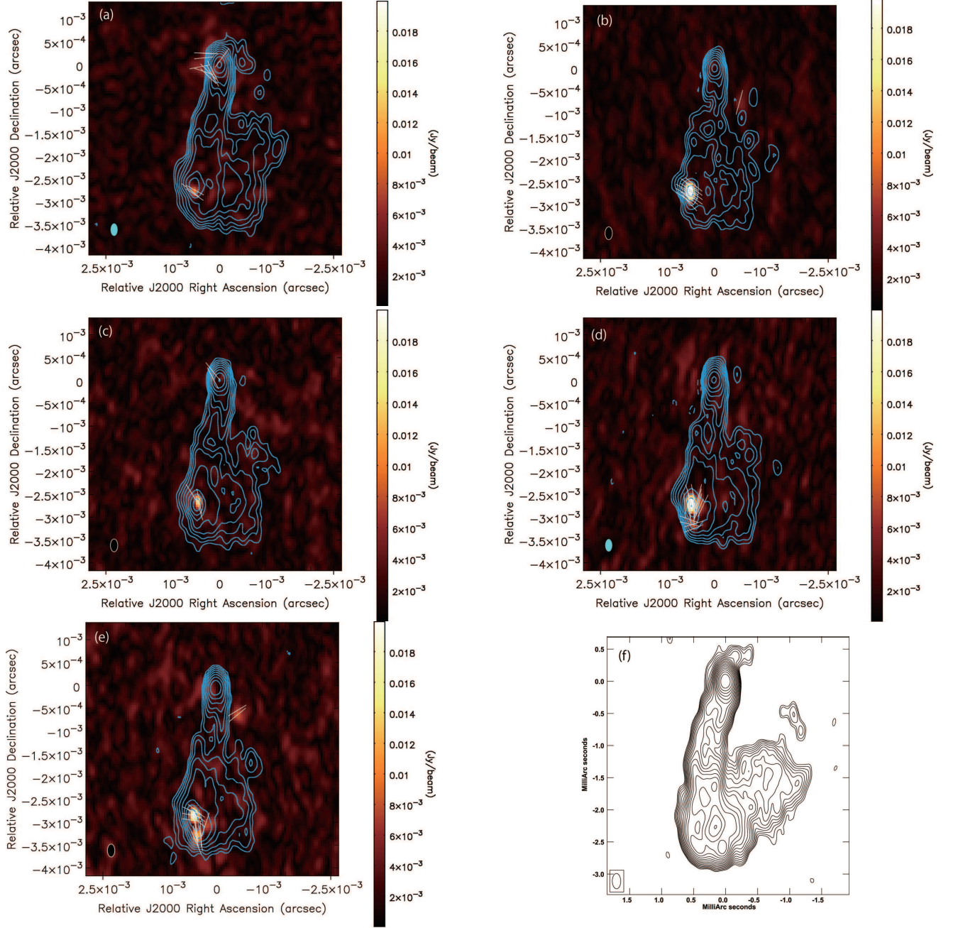
FIG. 1.— VLBA images of 3C 84 on (a) 2015 December 05, (b) 2016 January 01, (c) 2016 January 31, (d) 2016 March 18, and (e) 2016 April 22. Total intensity is indicated by cyan contours overlaid on the polarized intensity in color. Total intensity images are made by combining all four IFs while the polarized intensity is for IF1. The 1\sigma of the total intensities are 1.67 mJy, 5.56 mJy, 3.55 mJy, 3.99 mJy, and 4.44 mJy on 2015 December 05, 2016 January 01, 2016 January 31, 2016 March 18, and 2016 April 22, respectively. The contour levels are plotted at the level of (-1, 1, 2, 4, \dots, 2048) \times 3\sigma of each image. The polarization position angles are indicated by the white vectors, which are shown on the area where the polarized intensity is greater than 3\sigma of the polarized intensity images. The restoring beam size is (0.28 \times 0.16) mas at a position angle of 0^\circ . (f) The 43-GHz VLBA image of 3C 84 in 2013 January 24, which is the same image shown in Nagai et al. (2014).
