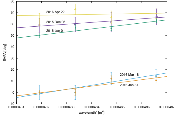
FIG. 2.— EVPA as a function of wavelengths square.
