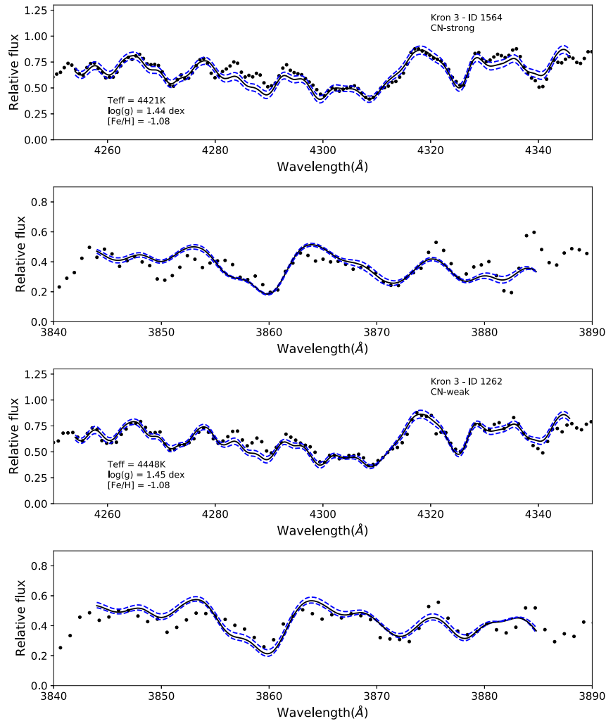
Figure 10. Spectrum synthesis of CH (first and third panels) and CN (second and fourth panels) features for stars ID 1564 (CN-strong) and ID 1262 (CN-weak). In all panels, the continuum normalized spectrum is represented by solid dots. First panel: the solid line represents the best abundance fit which has [C/Fe] = -0.90 , assuming [O/Fe] = +0.2 . The dashed blue lines show [C/Fe] values \pm 0.15 dex about the central value. Second panel: the solid line represents the best abundance fit with [N/Fe] = +0.15 and [C/Fe] = -0.9 , assuming [O/Fe] = +0.2 . The dashed blue lines show [N/Fe] values \pm 0.3 dex from the best fit. Third panel: the solid line represents the best abundance fit which has [C/Fe] = -0.70 assuming [O/Fe] = +0.2 . The dashed blue lines again show [C/Fe] values \pm 0.15 dex about the central value. Fourth panel: the solid line represents the best abundance fit with [N/Fe] = -0.55 and [C/Fe] = -0.70 , assuming [O/Fe] = +0.2 . The dashed blue lines show [N/Fe] values \pm 0.3 dex from the best fit. The observed spectra are identical to those shown in Fig. 9.
