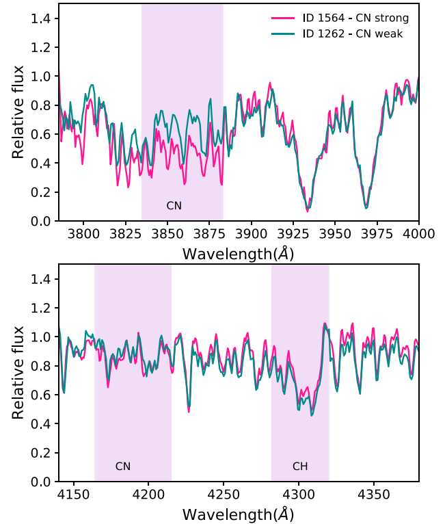
Figure 9. Continuum normalized spectra of target stars ID 1564 (CN-strong, pink) and ID 1262 (CN-weak, turquoise). The location of the CH, at \lambda \sim 4300 Å and the CN, at \lambda \sim 3883 Å and \lambda \sim 4215 Å bands are shown by the shaded regions. Star ID 1564 has S(3839) = 0.481 while for Star ID 1262 the value is 0.044 mag. Similarly, the W(G) values are 10.52 and 11.73 Å, respectively.
