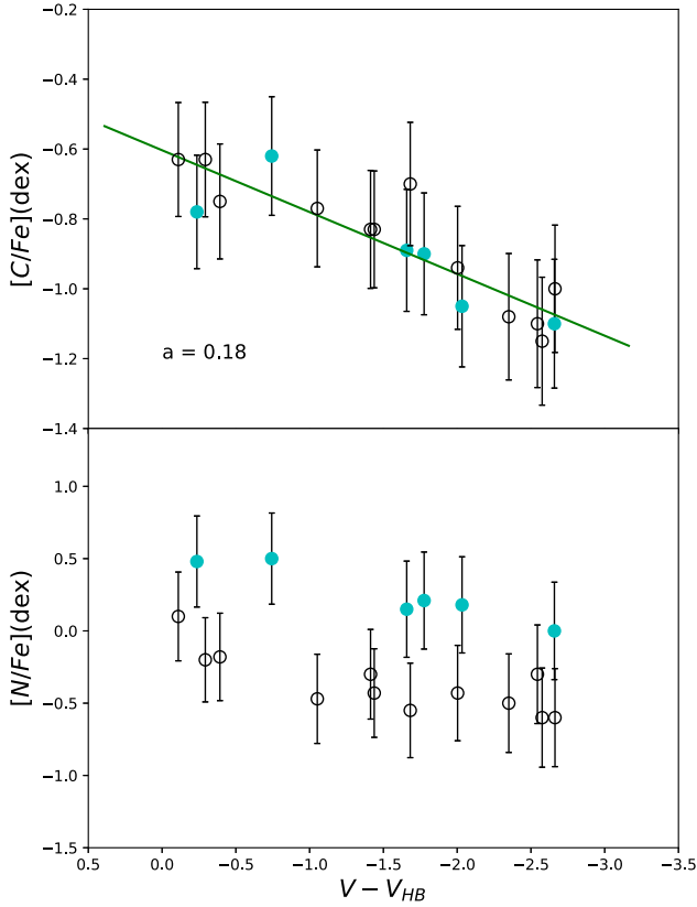
Figure 11. Upper panel: dependence of [C/Fe] on V magnitude for RGB members of the Kron 3. The green line represents the best fit and the corresponding slope value ‘a’ is given on the figure. Lower panel: dependence of [N/Fe] on V magnitude for RGB members of the Kron 3. In both panels filled and empty circles represent CN-strong and CN-weak stars, respectively.
