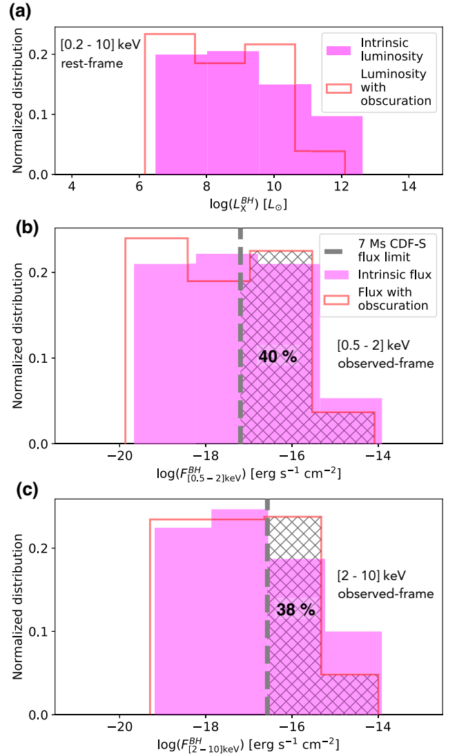
Figure 5. (a) Distribution of the intrinsic (the magenta histogram) and obscured (the red histogram) X-ray luminosities (integrated over the rest-frame soft + hard band, [0.2–10] keV) produced by the accreting BHs in the HyLIRG progenitors of high- z quasars. (b) and (c) Distributions of the intrinsic and obscured X-ray fluxes produced by the accreting BHs, in the observed-frame soft (panel b) and hard (panel c) X-ray bands. The grey dashed lines represent the flux limits of the 7 Ms CDF-S survey, i.e. F_{\text{CDF-S}} = 6.4 \times 10^{-18} \text{ erg s}^{-1} \text{ cm}^{-2} in the soft band, and F_{\text{CDF-S}} = 2.7 \times 10^{-17} \text{ erg s}^{-1} \text{ cm}^{-2} in the hard band. About 40 per cent (38 per cent) of the HyLIRGs population shows a detectable F_{\text{X}}^{\text{BH}} in the observed-frame soft (hard) band (hatched regions).
