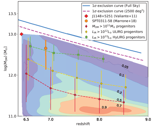
Figure 1. Density plot showing the M_{\text{DM}} distribution of DM haloes hosting massive progenitor galaxies ( M_{\text{DM}} > 10^{11} M_\odot ) of a J1148-like quasar host galaxy (the red point), in the redshift interval 6.4 < z < 9 . The density distribution is based on the total statistics of 10 different merger trees (see Section 2); the percentile levels are marked by the filled colour contours and labelled in the figure. The red dashed line and points represent the redshift evolution of the averaged M_{\text{DM}} of all massive progenitors ( M_{\text{DM}} > 10^{11} M_\odot ). The gold and green lines and points represent the redshift evolution of the average M_{\text{DM}} of haloes hosting massive progenitors with L_{\text{IR}} > 10^{12} L_\odot (ULIRGs) and L_{\text{IR}} > 10^{13} L_\odot (HyLIRGs), respectively. Error bars are indicative of the 1\sigma standard deviation calculated in equipartition redshift bins (the slight offset of the bins position for red, gold, and green points has been introduced to avoid overlapping and help visualization). The orange point represents the DM halo mass hosting the HyLIRG system SPT0311-58, at z = 6.9 (Marrone et al. 2018). The blue solid and magenta dashed lines represent the 1\sigma exclusion curves, i.e. the most massive haloes that are expected to be observable within the whole sky and a 2500 \text{deg}^2 area (the size of the SPT survey in which SPT0311-58 was identified), respectively, as a function of redshift (Harrison & Hotchkiss 2013; Marrone et al. 2018).
