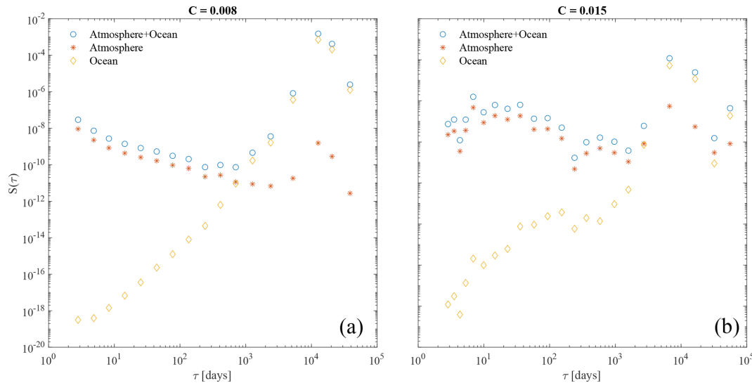
Figure 2. Spectral energy content S(\tau) of the different MIMFs as a function of their mean timescales \tau as in Eq. (7) for the full system (atmosphere+ocean, blue circles), only for the atmosphere (orange asterisks), and only for the ocean (yellow diamonds). Panel (a, b) refer to the two values of the friction coefficient, C = 0.008 and C = 0.015 , respectively.
