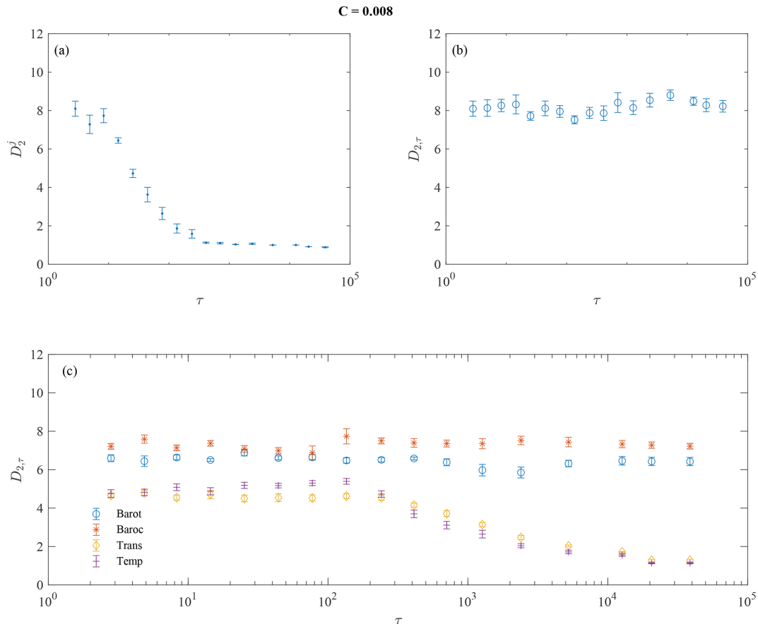
Figure 5. Multiscale correlation dimension D_{2,\tau} for C = 0.008 at different timescales \tau_j for different cases: (a) for each MIMF individually ( D_2^j ), (b) for reconstructions of MIMFs as in Eq. (12) ( D_{2,\tau} ), and (c) for reconstructions of MIMFs separately for each variable (barotropic modes – blue circles, baroclinic modes – orange asterisks, transport modes – yellow diamonds, and temperature modes – violet symbol). Each panel also shows the 95 % confidence intervals as error bars.
