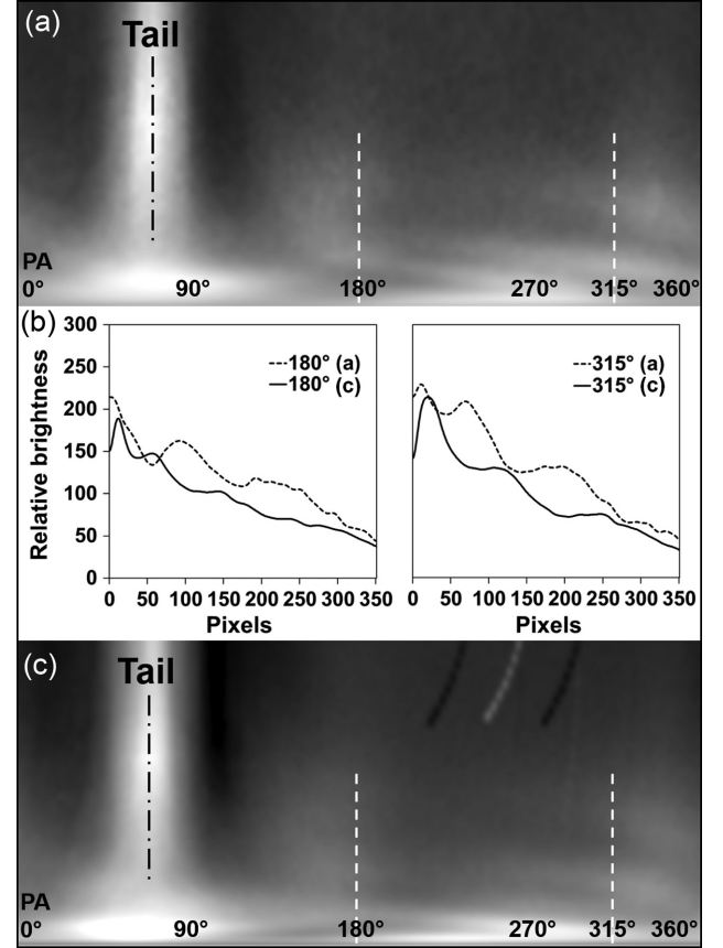
Figure 2. (a and c) Polar projections, centred on the optocentre of the false cometary nucleus, of two images of 2020 July 26, processed as in Fig. 1, taken with 1-h time interval. The projections show the development and expansion of the spirals. (b) The vertical photometric profiles at PA 180^\circ and 315^\circ provide the precise distance of each shell from the nucleus (in pixels).
