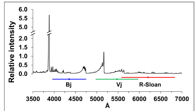
Figure 9. Two spectra were obtained on 2020 August 8 with the 1.22-m Galileo telescope at the Asiago Astrophysical Observatory with an exposure of 600 s and a resolution of 2.25 \text{ Å pixel}^{-1} . The two calibrated spectra were divided by a solar analogue to offset the contribution of the Sun, then co-added. The emissions of CN at 3880 Å and the C3 and C2 Swan-bands are very obvious. Below the spectrum, the respective central wavelength and FWHM of the Bj , Vj , and r -Sloan filters are shown.
