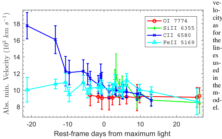
Figure 8. Line velocity evolution for Fe II \lambda 5169 , Si II \lambda 6355 , O I \lambda 7774 , and C II \lambda 6580 . The velocities are estimated from the absorption minima of the corresponding P Cygni profiles.
