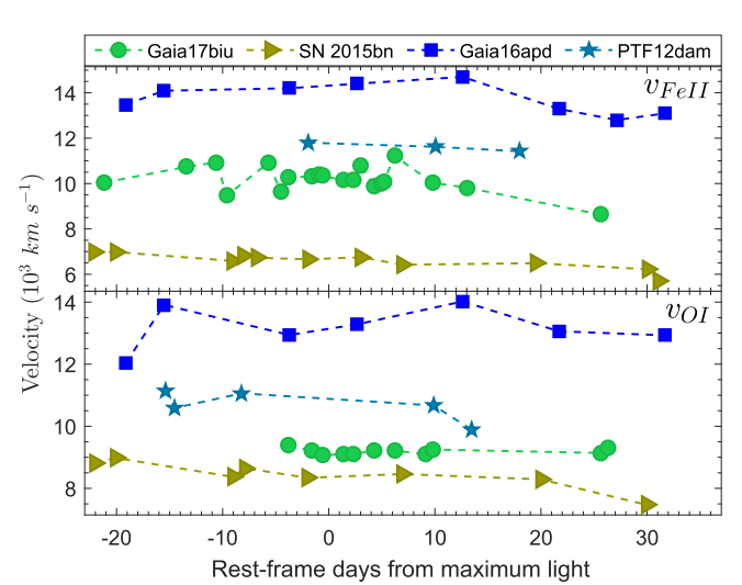
Figure 9. Fe II and O I \lambda 7774 line velocities of Gaia17biu as compared to SN 2015bn (Nicholl et al. 2016), Gaia16apd (Kangas et al. 2017), and PTF12dam (Nicholl et al. 2013). The Fe II velocities are measured using the \lambda 5169 line, except for SN 2015bn, where the \lambda 4924 line is used. In the case of PTF12dam, the Fe II \lambda 5169 velocities are presented in Nicholl et al. (2015b), while the O I velocities are measured from spectra (Nicholl et al. 2013).
