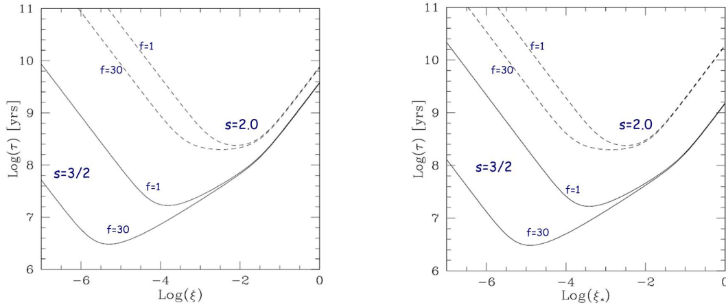
Figure 3. Acceleration time due to non-resonant acceleration as a function of \xi = \lambda_{mfp}/l_\lambda . Left panel is for \lambda_\lambda = M_o^{-3} L_o and right panel is for \lambda_\lambda = \max\{M_o^{-4} L_o, 2\pi/k_{cut}\} (see text). Turbulent cut-off scale is calculated both in the collisionless scenario ( k_{cut,s} Eqs.7 and 10, case (i), Sect. 3) and assuming k_{cut} = f k_{cut,s} (to mimic case (ii) in Sect.3). We show the case s=3/2 (solid) and 2.0 (dashed), other parameters being equal to Fig. 2.
