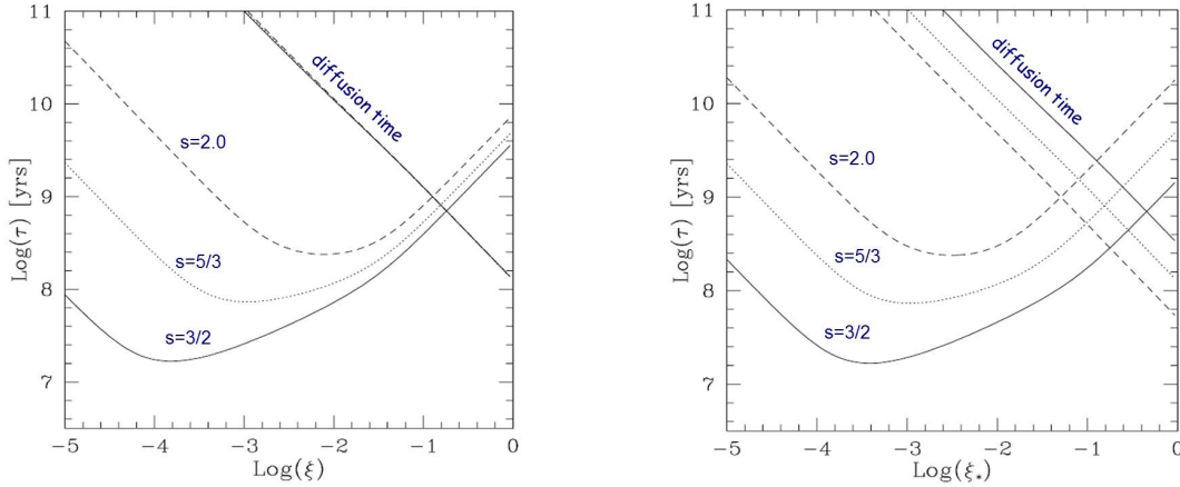
Figure 2. Acceleration time and (Mpc-scale) diffusion time due to non-resonant acceleration as a function of \xi = \lambda_{mfp}/l_\lambda . Left panel is for l_\lambda = M_o^{-3} L_o and right panel is for l_\lambda = \max\{M_o^{-4} L_o, 2\pi/k_{cut}\} (see text). The collisionless scenario (case (i), Sect. 3) is adopted to calculate the turbulent cut-off scale. In the calculations we assume \delta V = 750 km/s, and s = 3/2, 5/3, 2.0 , other parameters being equal to Fig.1.
