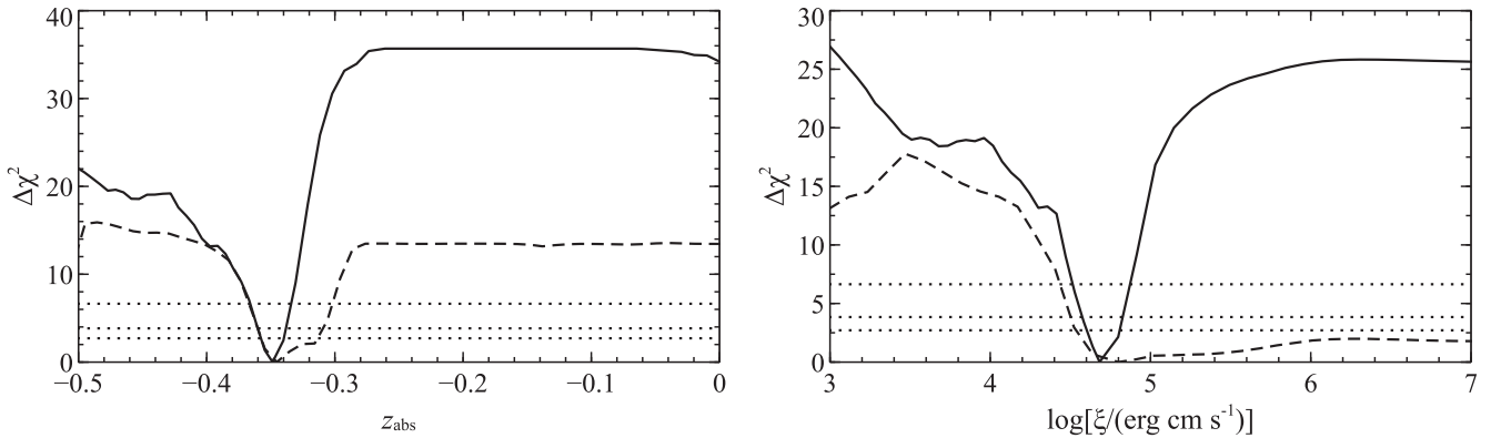
Figure 4. The \Delta\chi^2 confidence contours for the blueshift (left-hand panel, given in the rest frame of IRAS 00521–7054) and the ionization parameter (right-hand panel) of the highly ionized absorber. The horizontal dotted lines represent the 90, 95, and 99 per cent confidence levels for a single parameter of interest. The solid curves show the confidence contours for the full data set, and the dashed curves show the contours after excluding the 1.25–1.65 keV energy range to cut out the feature at \sim 1.5 keV.
