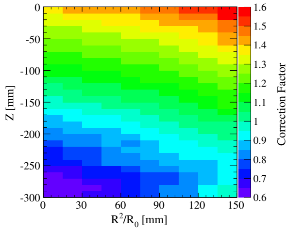
FIG. 3. Light correction map of XENON100 for high-energy alpha events, generated from ^{220}\text{Rn} and ^{216}\text{Po} decays. The radial parameter is defined according to the detector's radius, R_0 = 153 mm. Events at low (high) Z and low (high) radius R have the highest (lowest) light collection and thus a correction factor less (greater) than unity.
