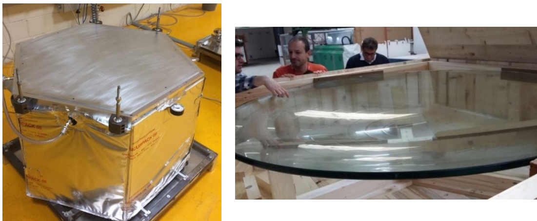
Figure 11. Mini-array mirrors production. Left: one of the primary segments being manufactured (courtesy of Media Lario srl). Right: secondary mirror substrate at Flabeg GmbH.
