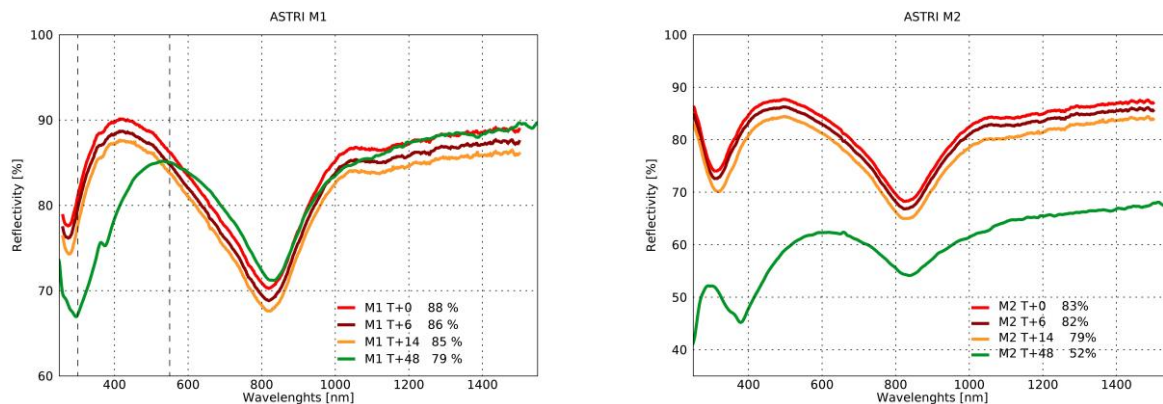
Figure 6. Reflectivity of M1 and M2 at different times. The reflectivity was measured after coating deposition and then 6, 14 and 48 months later.
