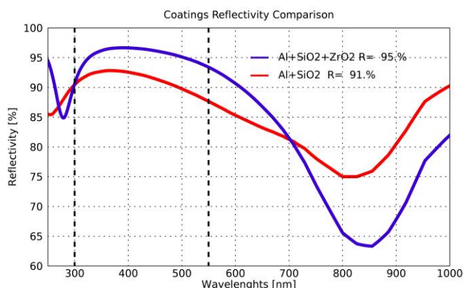
Figure 12. The reflectance of the coating of the ASTRI prototype mirrors ( \text{Al}+\text{SiO}_2 ) compared to that of the coating chosen for the ASTRI mini-array mirrors ( \text{Al}+\text{SiO}_2+\text{ZrO}_2 ).
