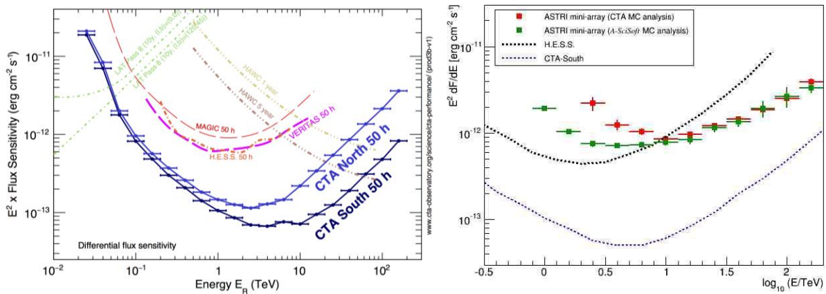
Figure 14. Left: The expected sensitivity of the CTA, achieved with cuts optimised for better low-energy response in the ASTRI case and for cuts optimised for a balanced performance in sensitivity and angular resolution for the full CTA South case, compared to existing IACT experiments, as well as the LAT instrument on board the Fermi satellite and the HAWC ground array [3]. Right: ASTRI mini-array (9 telescopes, relative distance \sim 250 m, square layout) differential sensitivity curves ( 5\sigma , 50 hours) achieved with the A-SciSoft MC analysis (green points) and with the CTA MC analysis. The differential sensitivities of CTA-South (blue line) and H.E.S.S. (black line) are also shown for comparison.
