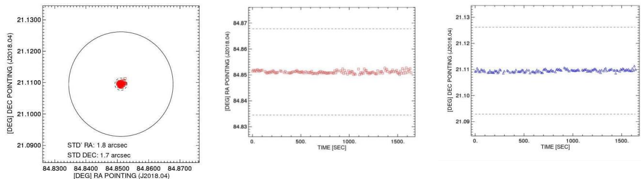
Figure 4. Pointing and tracking performance of the ASTRI telescope. Left: RA-DEC plot showing that the position of the telescope can be measured with an accuracy within the 7 arcsec (dashed circle) requested by the CTA requirement of post calibration astrometric accuracy. Center and right: RA and DEC plots versus time showing that ASTRI is well within the 1 arcmin (dashed lines) online astrometric accuracy requested by CTA.
