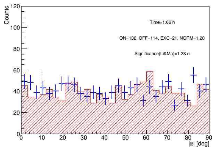
Figure 9. |\alpha| distributions of the Crab Nebula signal and background estimation from data taken in December 2017, after an 80% efficiency-based gamma/hadron discrimination parameter cut (in the whole energy range). The region between zero and the vertical dashed line (at 9 deg) represents the fiducial signal region. See [20] for further details.
