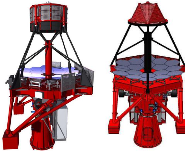
Figure 13. Design of the ASTRI Telescope mechanical structure. Left: the ASTRI prototype. Right: the consolidated design (courtesy of GEC)
