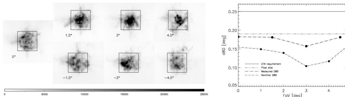
Figure 5. Left: PSF of ASTRI SST-2M telescope across the focal plane. Cherenkov camera pixel size (7x7 mm) is over-plotted for each PSF. Right: Comparison of D80 (diameter of the circle corresponding to an encircled energy of 80%) as a function of field angle (off-axis) between its ideal (dot-dashed curve) and measured at ASTRI SST-2M (dashed curve) values. SiPM pixel size (dashed horizontal line) and CTA requirement (solid horizontal line) are also shown for reference.
