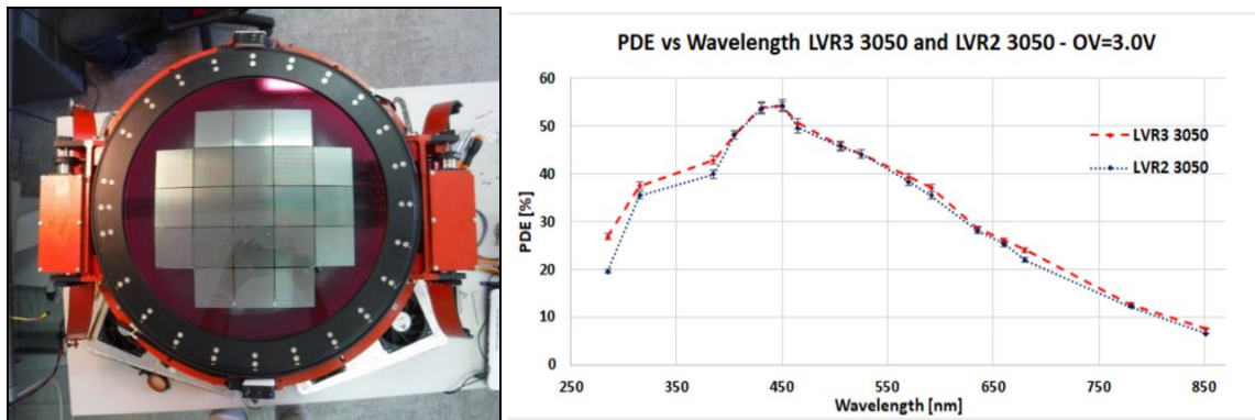
Figure 3. Left: the ASTRI prototype camera integrated in the laboratory. Right: Photo Detection Efficiency of last generation Hamamatsu LVR2 and LVR3 SiPM sensors.
