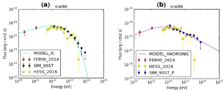
Figure 15. Simulated spectra of the SNR RCW 86 observed with the ASTRI mini-array in case of (a) leptonic (cyan line) or (b) hadronic (magenta line) mechanism of the gamma-ray origin dominates. ASTRI simulated data points are in the (a) black and (b) blue colors. For H.E.S.S. observational data points see [26] and for Fermi-LAT [25].
