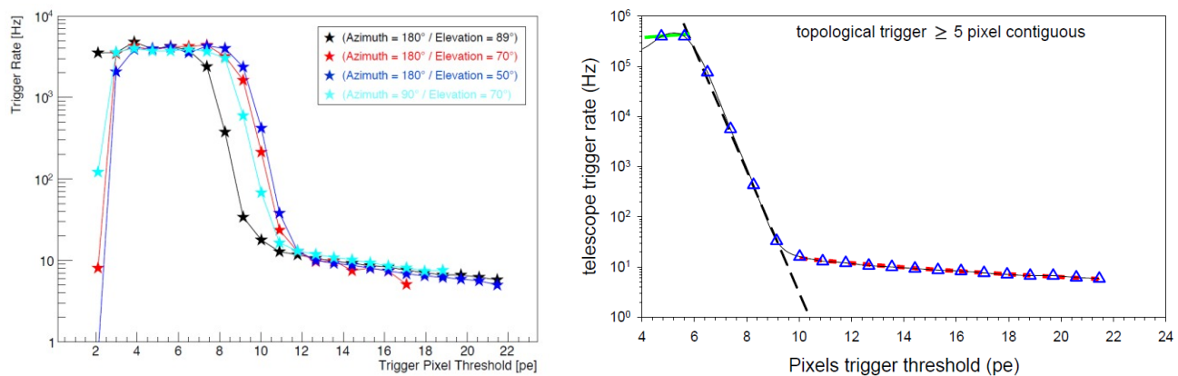
Figure 8. Trigger rate as a function of the trigger threshold in photoelectrons. Left: scans at different telescope pointing [20]. Right: trigger rate obtained pointing at zenith and corrected for dead time. Also shown are the trigger rate saturation (green line) and the random coincidence rates (black dashed line) induced by the NSB diffuse light. The red dashed line represents a power-law fit to the data points for thresholds greater than 10 pe [17].
