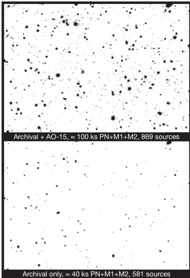
Figure 10. Top – Background-subtracted, smoothed, and co-added PN+MOS image in the 0.5–10 keV band for a 0.8 \times 0.6 \text{ deg}^2 region centred at RA = 35.580°, Dec. = -4.965^\circ . This image is created using both archival data and the new AO-15 data, and a total of 869 sources are detected in this region. Bottom : Same as the top image but only the archival data are included. The two images are matched in colour scale. In the Liu et al. (2016) catalogue, only 581 sources can be found in this region. The typical vignetting-corrected exposure times are shown at the bottom of both panels. The exposure time of the full survey region is shown in Fig. 3.
