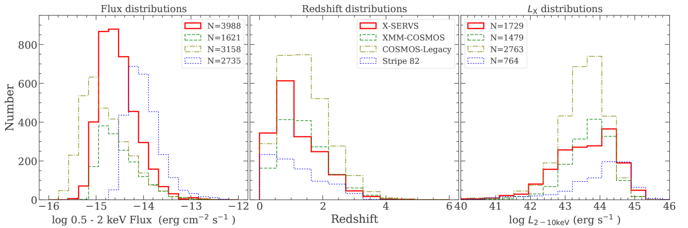
Figure 21. 2\text{--}10\text{keV} comparison between this work (solid red line), XMM-COSMOS (green dashed line), COSMOS-Legacy (brown dash-dotted line), and Stripe 82–X (blue dotted line). Distributions shown in panels from left to right are: 0.5\text{--}2\text{ keV} flux, redshift, and \log L , respectively. The left-hand panel shows the distribution of soft-band fluxes for the soft-band detected sources in each catalogue; no redshift information is required. The number of the soft-band sources is listed in the left-hand panel. For the middle and right-hand panels, the histograms are for the subset of sources with redshift measurements (regardless of the detection bands), with source numbers marked in the right-hand panel.
