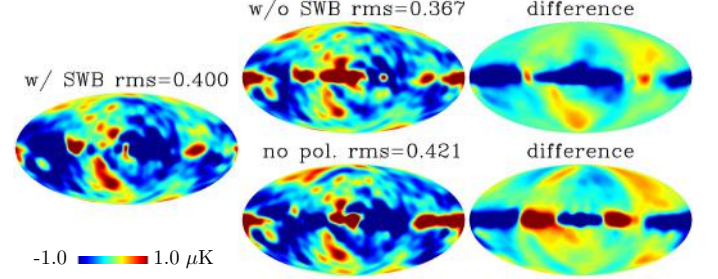
Fig. 9: 217-GHz Q maps cleaned using the 353-GHz map built with the SWBs (left), without the SWBs (top centre), and with the SWBs but with a polarization efficiency taken to be zero (bottom centre). The differences (right two maps) leave quadrupole terms of amplitude smaller than 1 \mu\text{K} .
