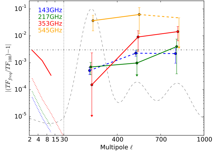
Fig. 41: Transfer function ratio, referred to 100 GHz, for various multipoles. For \ell = 2 –30, the solid red line is the measured 353-GHz empirical SRoll time TF. The red dotted line shows an upper limit on the 353-GHz residuals after correction, while blue and green dotted lines show an estimate of the residuals at 143 and 217 GHz. The TF for \ell = 30 –1000 is estimated from CMB anisotropies on the first three acoustic peaks (with negative values displayed by dashed lines). The grey dashed line is a CMB power spectrum, showing the position of the first three acoustic peaks.
