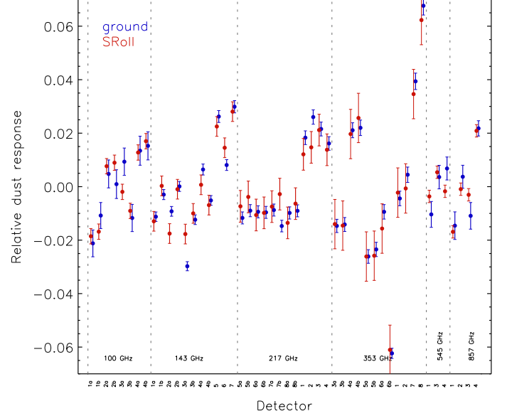
Fig. 42: Recovery of dust leakage coefficients from the ground measurements (in blue) and those from SRO11 (in red).
