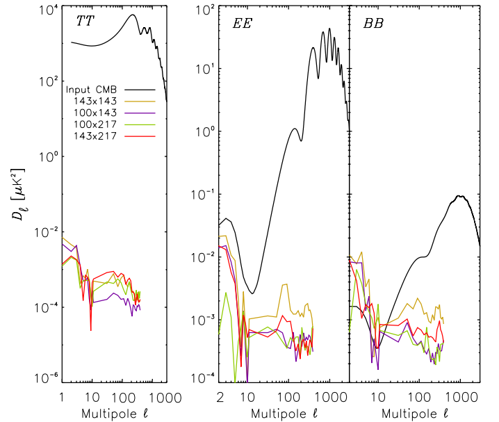
Fig. 51: Cross-spectra between the three CMB channels, showing the non-linear distortion of strong signals (not corrected in SRoll). The auto-spectrum of the lowest noise 143-GHz channel is shown to illustrate the reduction of the systematic level brought by the use of cross-spectra. At \ell > 300 , quantization noise generates a rise not related to this test; hence that range of multipoles is not shown.
