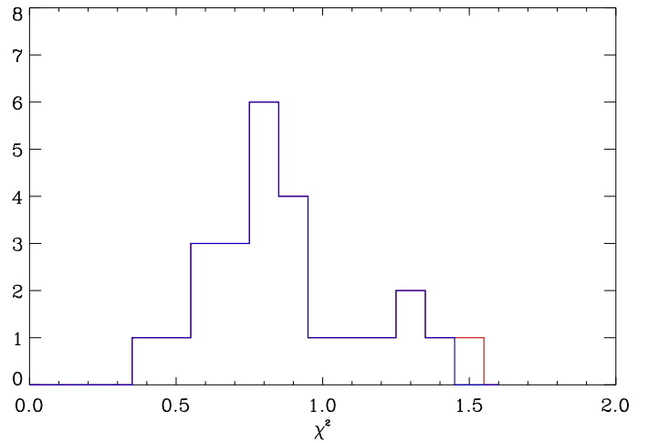
Fig. 3: Histogram the \chi^2 distribution for the maps in which a set of 1000 consecutive pointing periods has been removed (see text). The red line shows the \chi^2 for the last block of pointing periods removed.
