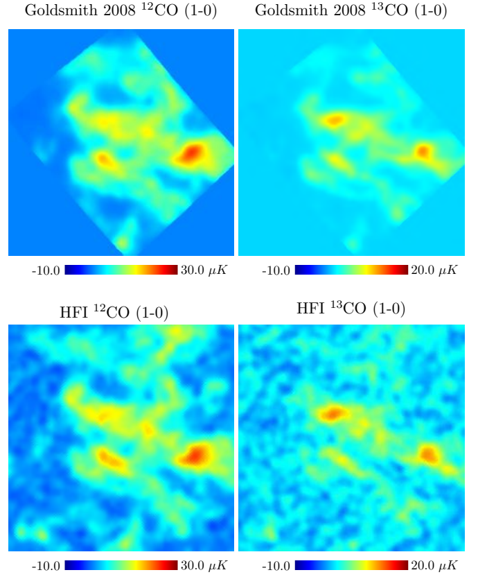
Fig. 6: Top panel : two ground-based radio astronomy maps, centred on (173^\circ 0, -16^\circ 0) in Galactic coordinates, at ^{12}\text{CO} and ^{13}\text{CO} in the Taurus region. Bottom panel : HFI ^{12}\text{CO} and ^{13}\text{CO} maps extracted by SRoll.
