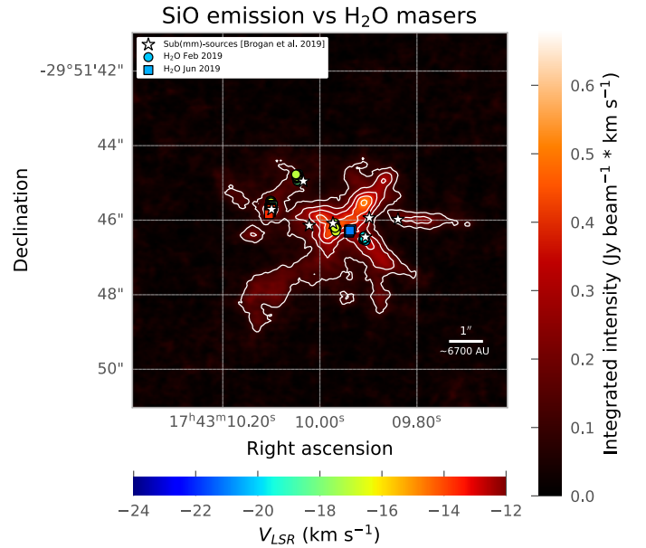
Fig. 10. 22 GHz water maser spot map overplotted on the moment 0 map (integrated over the velocity span of -40 to 3.2 km s -1 ) of the SiO J = 5-4 emission obtained with ALMA. The contour levels are [1, 2, 3, 4, 5] \times 0.1 Jy beam -1 km s -1 .
