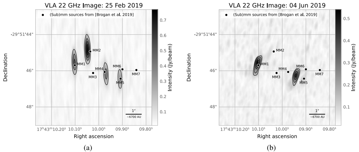
Fig. 5. 22 GHz \text{H}_2\text{O} maser emission detected in G358.93-0.03 with the VLA during (a) epoch I and (b) epoch II.
