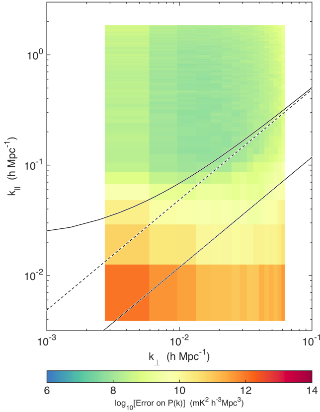
FIG. 7. By including both residual foregrounds and noise in \mathbf{C} , our model for the covariance, we can calculate the expected variance on each band power in \hat{\mathbf{p}} , which we show here. We see more variance at high (and also very low) k_{\perp} where we have few baselines. We also see high variance at low k_{\parallel} consistent with foregrounds. We see the strongest foregrounds at low k_{\perp} , which implies that the residual foregrounds have a very strong diffuse component that that we have much to gain from better diffuse models to subtract. We also also see that foreground-associated variance extends to higher k_{\parallel} at high k_{\perp} , which is exactly the expected effect from the wedge. Both these observations are consistent with the structure of the eigenmodes we saw in Figure 1. Because we have chosen a normalization of \hat{\mathbf{p}} such that the \text{Cov}(\hat{\mathbf{p}}) is diagonal, this is a complete description of our errors. Furthermore, it means that the band powers form a mutually exclusive and collectively exhaustive set of measurements.
