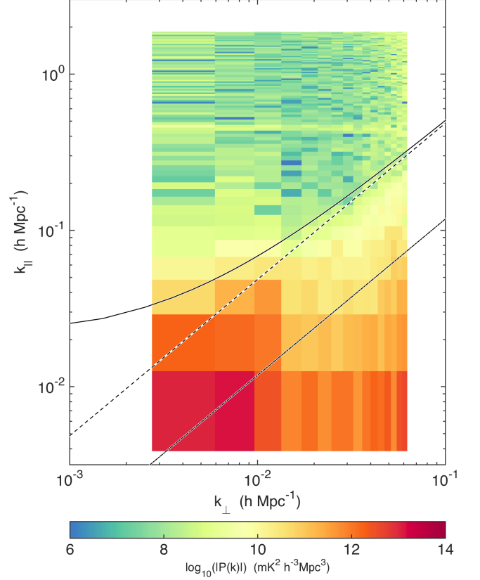
FIG. 5. Our power spectrum clearly exhibits the typical EoR window structure with orders-of-magnitude suppression of foregrounds in the EoR window. Here we plot our estimates for |P(k_\perp, k_\parallel)| for the full instrumental bandwidth, equivalent to the range z = 6.2 to z = 7.5 . Overplotted is the wedge from Equation 1 corresponding to the first null in the primary beam (dash-dotted line), the horizon (dashed line), and the horizon with a relatively aggressive 0.02 h \text{ Mpc}^{-1} buffer (solid curve). In addition to typical foreground structure, we also see the effect of noise at high and very low k_\perp where baseline coverage is poor. We also clearly see a line of power at constant k_\parallel \approx 0.45 h \text{ Mpc}^{-1} , attributable to miscalibration of the instrument’s bandpass and cable reflections [70].
