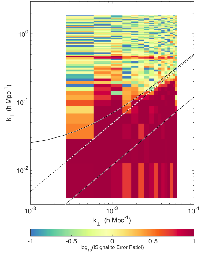
FIG. 8. The foregrounds’ wedge structure is particularly clear when looking at the ratio of our measured power spectrum to the modeled variance, shown here. Though the variance in foreground residual dominated parts of the k_{\perp} - k_{\parallel} plane are elevated (see Figure 7), we still expect regions with signal to error ratios greater than one. This is largely due to the fact that we choose not to subtract a foreground bias for fear of signal loss. This figure shows us most clearly where the foregrounds are important and, as with Figure 6, it shows where we can hope to do better with more integration time and where we need better calibration and foreground modeling to further integrate down.
