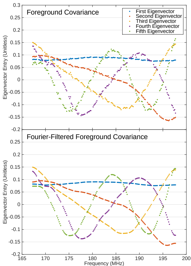
FIG. 3. The foreground covariance we estimate from our limited data set is still very noisy and we run the risk of overfitting the noise in our measurements if we take it at face value. In the top panel, we plot the eigenvectors corresponding to the five largest eigenvalues of \hat{\mathbf{C}}^{\text{FG}} for a mode in the annulus centered on k_{\perp} \approx 0.010 h \text{ Mpc}^{-1} . In the bottom panel, we show dominant eigenvectors of the Fourier-filtered covariance. As expected, they resemble the first five Fourier modes. The missing data every 1.28 MHz is due to channels flagged at the edge of the coarse bandpass of the MWA’s polyphase filter bank—the most difficult part of the band to calibrate.
