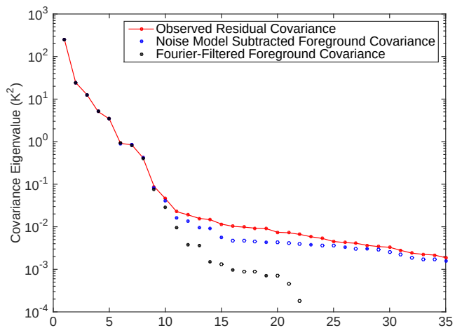
FIG. 4. This figure shows the evolution of the eigenvalues of our estimated foreground covariance matrix for a mode in the annulus corresponding to k_{\perp} \approx 0.010 h \text{ Mpc}^{-1} at each of the first three stages of covariance estimation. First we calculate a sample covariance matrix from the residual data cubes (shown in red). Next we subtract our best guess as to the part of the diagonal of that matrix that originates from instrumental noise, leaving the blue dots (open circles are absolute values of negative eigenvalues). Then we filter out modes in Fourier space along the line of sight that we think should be noise dominated, leaving the black dots. Finally, we project out the eigenvectors associated with eigenvalues whose magnitude is smaller than the largest negative eigenvalue, since those are likely due to residual noise. What remains is our best guess at the foreground covariance in an annulus and incorporates as well as possible our prior beliefs about its structure.
