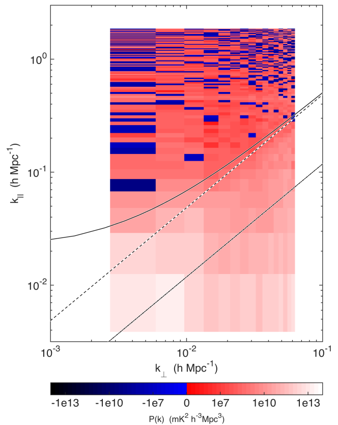
FIG. 6. By using an estimator of the power spectrum with uncorrelated errors between bins, we can see that most of the EoR window is noise dominated in our power spectrum measurement. Here we show the inverse hyperbolic sine of the power spectrum, which behaves linearly near zero and logarithmically at large magnitudes. Because we are taking a cross power spectrum between two data cubes with uncorrelated noise, noise dominated regions are equally likely to have positive power as negative power. Since we do not attempt to subtract a foreground bias, foreground contaminated regions show up as strongly positive. That includes the wedge, the bandpass line at k_{\parallel} \approx 0.45 h \text{ Mpc}^{-1} (see Figure 5), and some of the EoR window at low k_{\perp} and relatively low k_{\parallel} , consistent with the suprahorizon emission seen in [26].
