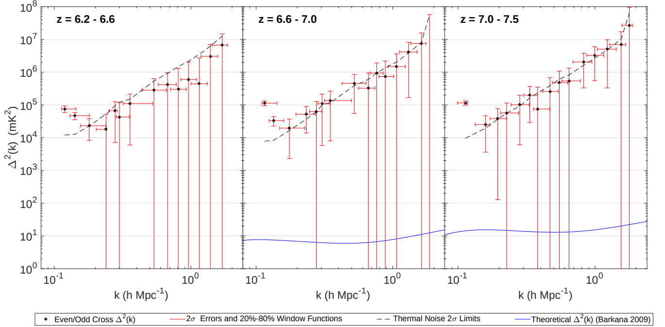
FIG. 9. Finally, we can set confident limits on the 21 cm power spectrum at three redshifts by splitting our simultaneous bandwidth into three 10.24 MHz data cubes. The lowest k bins show the strongest “detections,” though they are attributable to suprahorizon emission [26] that we expect to appear because we only cut out the wedge and a small buffer ( 0.02 h \text{ Mpc}^{-1} ) past it. We also see marginal “detections” at higher k which are likely due to subtle bandpass calibration effects like cable reflections. The largest such error, which occurs at bins around k_{\parallel} \sim 0.45 h \text{ Mpc}^{-1} and can be seen most clearly in Figure 8, has been flagged and removed from all three of these plots. Our absolute lowest limit requires \Delta^2(k) < 3.7 \times 10^4 \text{ mK}^2 at 95% confidence at comoving scale k = 0.18 h \text{ Mpc}^{-1} and z = 6.8 , which is consistent with published limits [8, 12–15]. We also include a simplistic thermal noise calculation (dashed line), based on our observed system temperature. Though it is not directly comparable to our measurements, since it has different window functions, it does show that most of our measurements are consistent with thermal noise. For comparison, we also show the theoretical model of [72] (which predicts that reionization ends before z = 6.4 ) at the central redshift of each bin. While we are still orders of magnitude away from the fiducial model, recall that the noise in the power spectrum scales inversely with the integration time, not the square root.
