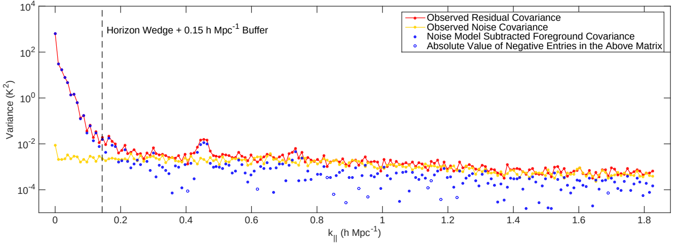
FIG. 2. Examining the diagonal elements of the observed residual and inferred foreground covariance matrices in Fourier space reveals the effectiveness of subtracting model for the noise covariance. In red, we plot the observed residual covariance, which contains both foregrounds and noise. As a function of k_{\parallel} , the two separate relatively cleanly—there is a steeply declining foreground portion on the left followed by a relatively flat noise floor on the right. The theory that the righthand portion is dominated by noise is borne out by the fact that it so closely matches the observed noise covariance, inferred lines of sight of \mathbf{x}_1 - \mathbf{x}_2 , which should have only noise and no sky signal at all. The regions where they differ significantly, for example at k_{\parallel} \sim 0.45 \text{ h Mpc}^{-1} , are attributable to systematic effects like the MWA’s coarse band structure that have not been perfectly calibrated out. For the example covariances shown here (which correspond to a mode in the annulus at k_{\perp} \approx 0.010 \text{ h Mpc}^{-1} ), we can see that subtracting a properly projected noise covariance removes most of the power from the noise-dominated region, leaving only residual noise that appears both as negative power (open blue circle) and as positive power (closed blue circles) at considerably lower magnitude.
