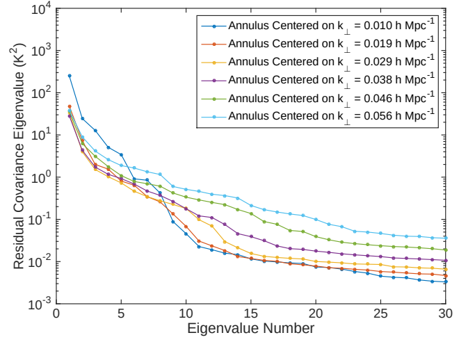
FIG. 1. The evolution of the wedge with k_\perp motivates us to model foregrounds separately for discrete values of k_\perp . In this plot of the thirty largest eigenvalues of the observed residual covariance (which should include both noise and foregrounds) sampled in six concentric annuli, we see steeper declines toward a noise floor for the inner annuli than the outer annuli. This is consistent with the expected effect of the wedge—higher k_\perp modes should be foreground-contaminated at higher k_\parallel .
