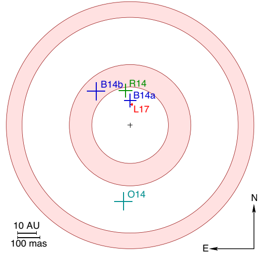
Figure 1. Diagram of the HD 169142 system. The red parts represent the two rings and the white parts are the gaps. The crosses represent the positions of the point-like structures discovered by Biller et al. (2014, B14b for the structure discovered with MagAO and B14a for the one detected with NaCo), Reggiani et al. (2014, R14) and Osorio et al. (2014, O14). We also show the structure around 100 mas detected with SPHERE in this work (L17, see Section 5). The dimension of the crosses represents the error bars (on scale), except for B14b and O14, where the error bars are given arbitrarily. The inclination of the disc is not shown in this diagram.
