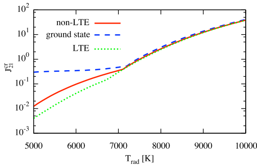
Fig. 1. The dependence of J_{21}^{cr} on the temperature of the blackbody spectra. The calculations are done with the different prescriptions for the population of the H_2^+ vibrational levels.
