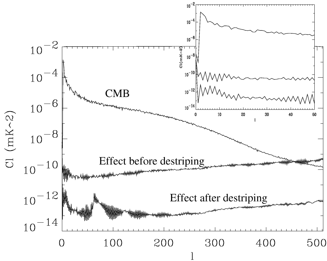
Figure 9 – Power spectra of the effect before and after destripping at 30 GHz (coupled scenario). A typical CMB power spectrum is plotted for comparison
