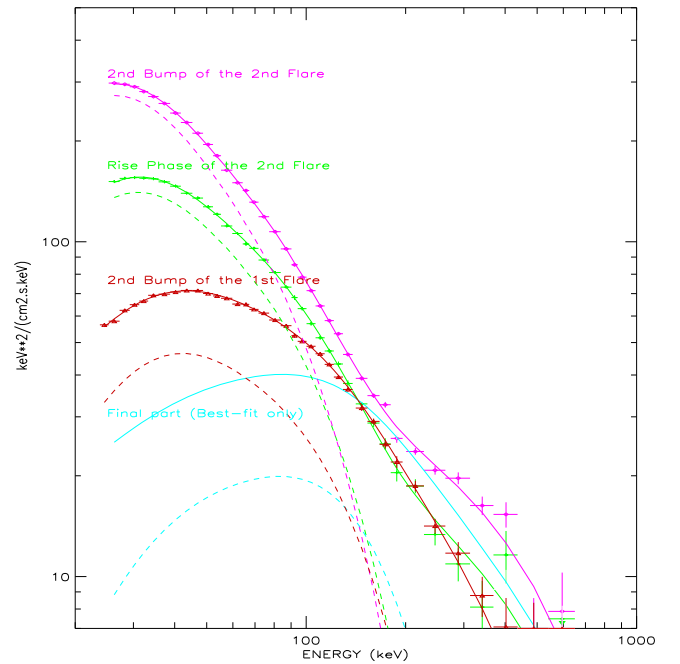
Figure 4. Comparison of hard and soft “states” of V404 Cyg as observed during Rev 1557. The three brightest spectra illustrate the source evolution between the second bump of the first flare, and RP and second bump of the second flare. Spectrum averaged over the last (hardest) part of the second flare is shown for comparison. Dashed lines correspond to the respective Compton components and illustrate their role in the source evolution.
