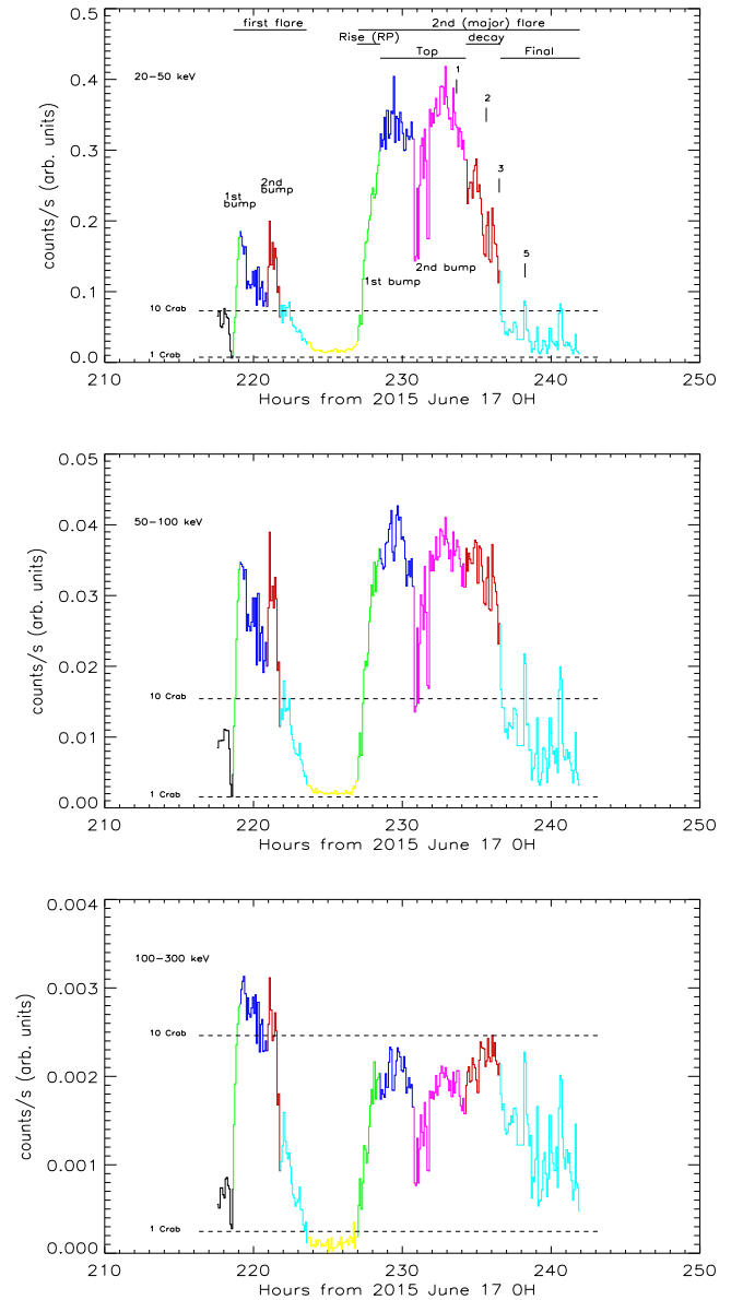
Figure 1. V404 Cyg light curve along Rev. 1557, for E = [20-50 \text{ keV}] , [50-100 \text{ keV}] and [100-300 \text{ keV}] from top to bottom. Time bins = 300 s. The data used to create this figure are available.
