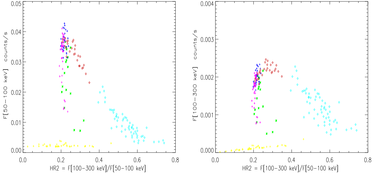
Figure 3. HID at higher energy, for the second flare only. F2 vs. HR2 = F3/F2 (left) and F3 vs. HR2 (right). The data used to create this figure are available.
