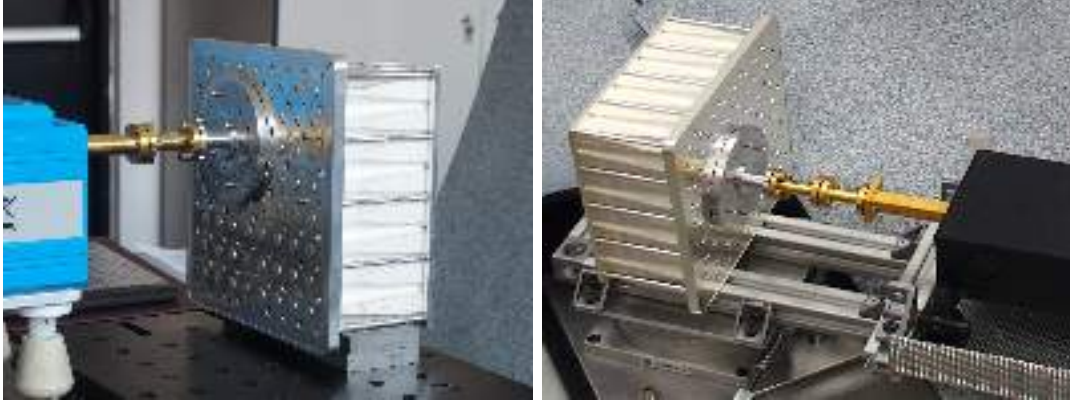
Figure 14. Left: detail of the adapter cascade used in the 110–170 GHz measurements. After the VNA golden millimeter extension where the TRL calibration plane is defined, there is a golden rectangular to circular waveguide taper. The golden taper is connected to the horn array by means of silver flange adapter. Right: detail of the adapter cascade used in the 170–260 GHz measurements. A rectangular taper from WR4.3 to WR06 is attached to the VNA golden waveguide millimeter extension (TRL calibration plane). After that, the same components of the lower band set-up is used.
