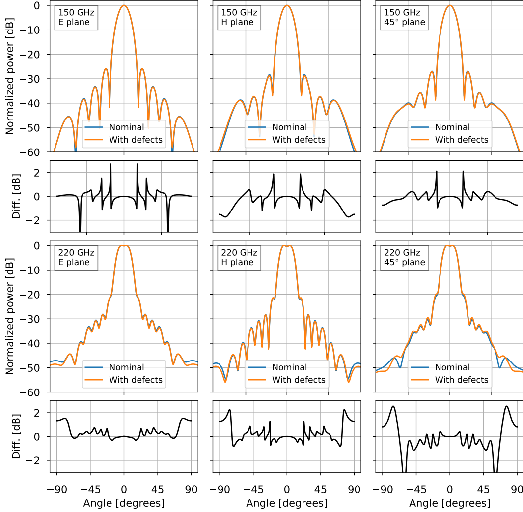
Figure 10. Impact of defects on the co-polar radiation patterns. The black line in the bottom panel shows the difference between the two beam patterns. The top plots refer to 150 GHz simulations, the bottom plots refer to 220 GHz simulations.
