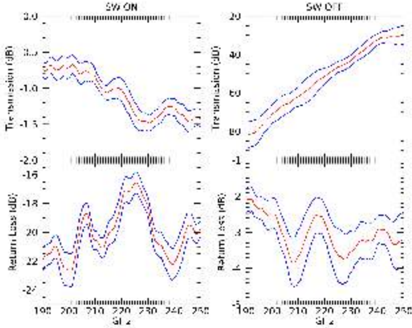
Figure 26. Measured insertion loss (top) and return loss (bottom) of the switch prototype in the band 190–250 GHz. Left: Switch ON. Right: Switch OFF. 1- \sigma confidence bands are plotted in blue.
