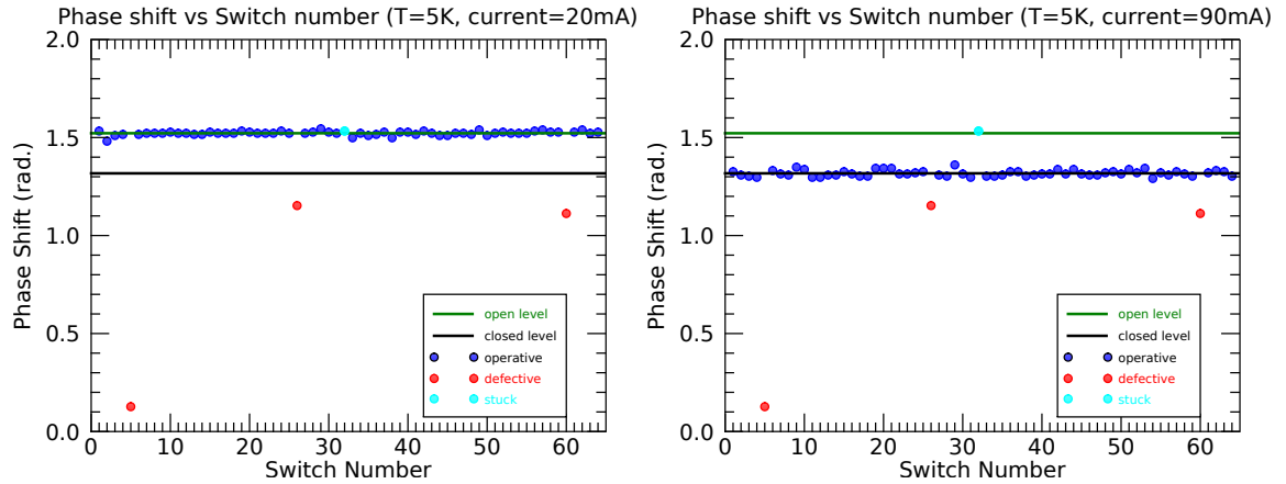
Figure 30. Phase between voltage and current measured by XOR algorithm. Left: shutters in open position Right: shutters in closed position. Switch n. 1 was operative at 5 K. N. 5, 26 and 60 were defective and n. 32 was stuck open.
