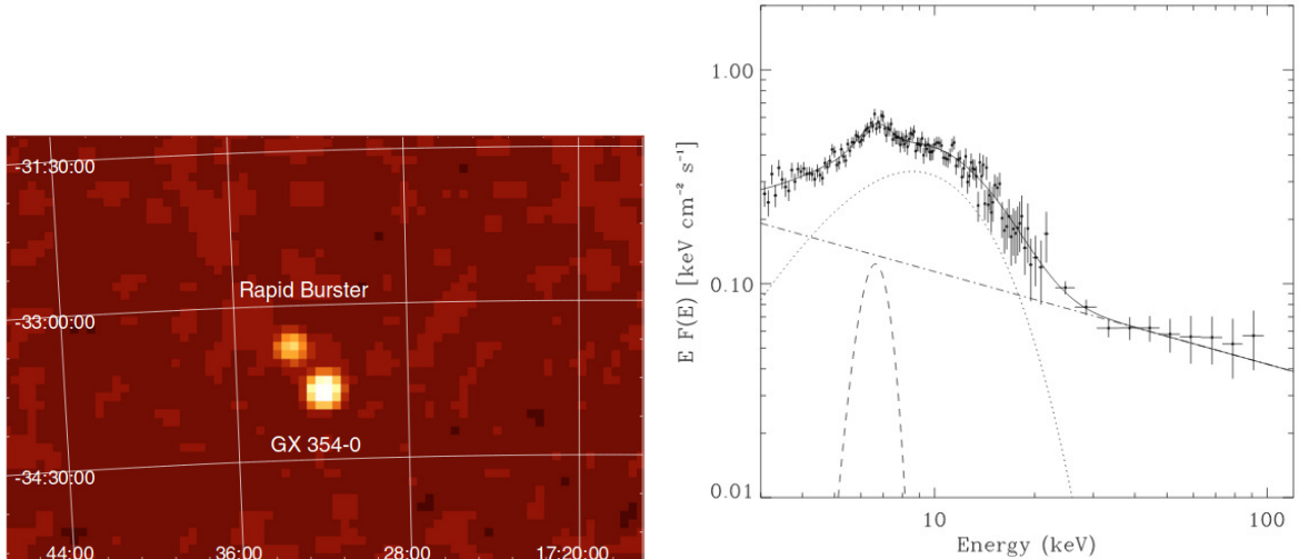
Figure 7: Left panel : IBIS/ISGRI 20–40 keV image of the Rapid Burster, for the first time resolved from the nearby 4U 1728–34=GX 354–0. Right panel : JEM-X and IBIS/ISGRI spectrum of the source. The hard tail in a soft spectral state is clearly visible. (From Falanga et al. 2004)
