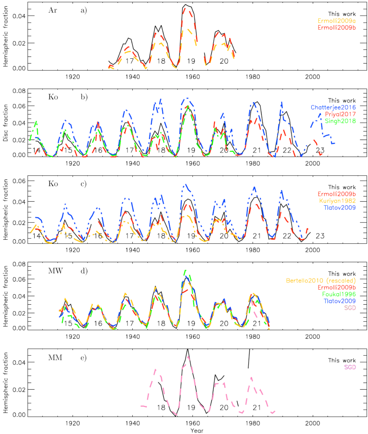
Fig. 11. Comparison of the plate areas derived here (black) to other published series based on the same datasets: (a) Ermolli et al. (2009a, yellow) and Ermolli et al. (2009b, red) for Ar data; (b) Chatterjee et al. (2016, blue), Priyal et al. (2017, red), and Singh et al. (2018, green) for Ko areas in disc fractions; (c) Ermolli et al. (2009b, red), Kuriyan et al. (1982, yellow), and Tlatov et al. (2009, blue) for Ko areas in fractions of a hemisphere; (d) Bertello et al. (2010, yellow), Ermolli et al. (2009b, red), Foukal (1996, green), Tlatov et al. (2009, blue), and SGD (pink) for MW data; (e) SGD (pink) for MM data. The curves are annual median values. All panels except b) are in fractions of hemisphere corrected for projection effects. The numbers under the curves denote the conventional SC numbering.
