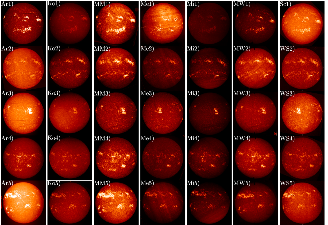
Fig. 1. Raw Ca II K density images from the Arcetri (Ar), Kodaikanal (Ko), McMath-Hulbert (MM), Meudon (Me), Mitaka (Mi), Mt Wilson (MW), Schauinsland (Sc), and Wendelstein (WS) observatories (Sc and WS are shown in a single column due to their low number of images). Each row shows observations from the different archives taken on roughly the same day, except for Me1. The dates of the observations are (from top to bottom): 09/12/1959 (17/11/1893 for Me), 01/03/1968 (29/02/1968 for Me), 01/08/1968 (30/07/1968 for Me and WS), 05/09/1968 (06/09/1968 for WS), and 18/03/1969 (17/03/1969 for Me and WS). All images are normalised to the range of values within the disc and are compensated for ephemeris.
