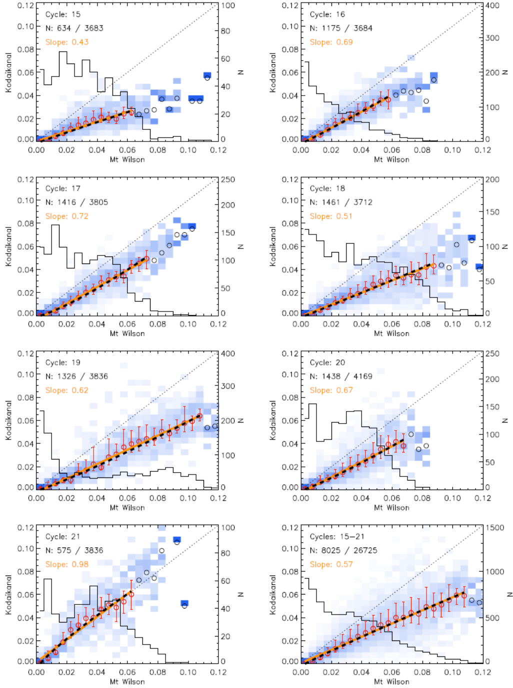
Fig. 7. Probability distribution functions (PDF) for fractional disc coverage by plate derived from Ko data, within area bins of 0.005, as a function of the disc fractions from MW for the same days. The PDF are colour-coded with white being 0 and bright blue 1. The Ko series is taken as the reference for this particular representation. Circles denote the average value within each column. For columns with less than 20 days of data these circles are shown in black, otherwise in red. We also show the asymmetric 1\sigma interval for each column. Two different fits to the average values are over-plotted; a linear fit (yellow) and a power law fit (black). The number of days included in each column is over-plotted with a solid black line (see right-hand axis). The dotted black line has a slope of unity and represents the expectation value. Each panel shows the PDF matrix for a given SC, while the lower right panel is for the whole interval of overlap between the compared series. The number of overlapping days used to construct each matrix (N) and the total number of days within each time interval is written in the plots. The slope of the linear fit is also given.
