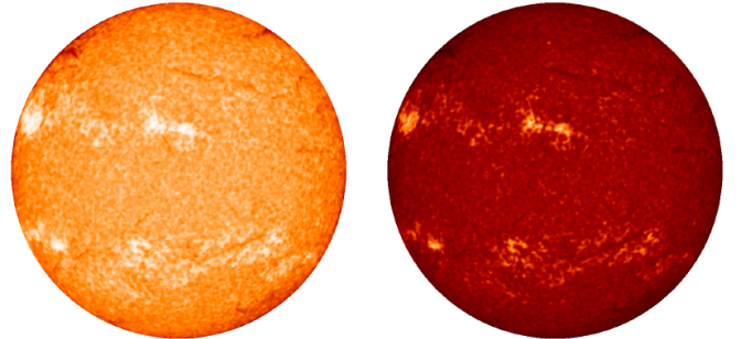
Fig. A.2. Me observation taken on 30/10/1998. Left: image converted to density values automatically by the scanner; right: image after our correction.
