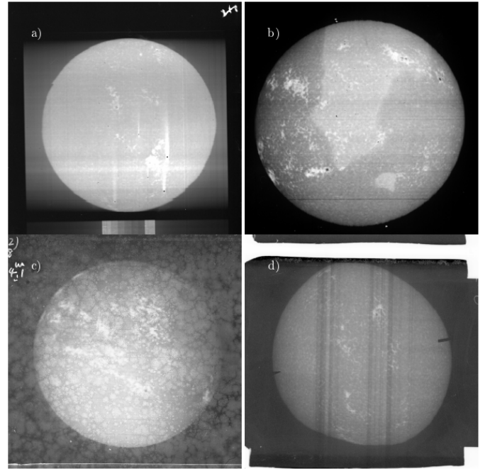
Fig. A.1. Examples of historical observations that were excluded from this study. Shown are the raw density images. The plotted examples were taken at the: (a)) Arcetri (21/03/1941), (b)) Kodaikanal (18/03/1990), (c)) Mitaka (11/04/1948), and (d)) Mt Wilson (17/01/1973) observatories. The images are not compensated for solar ephemeris.
