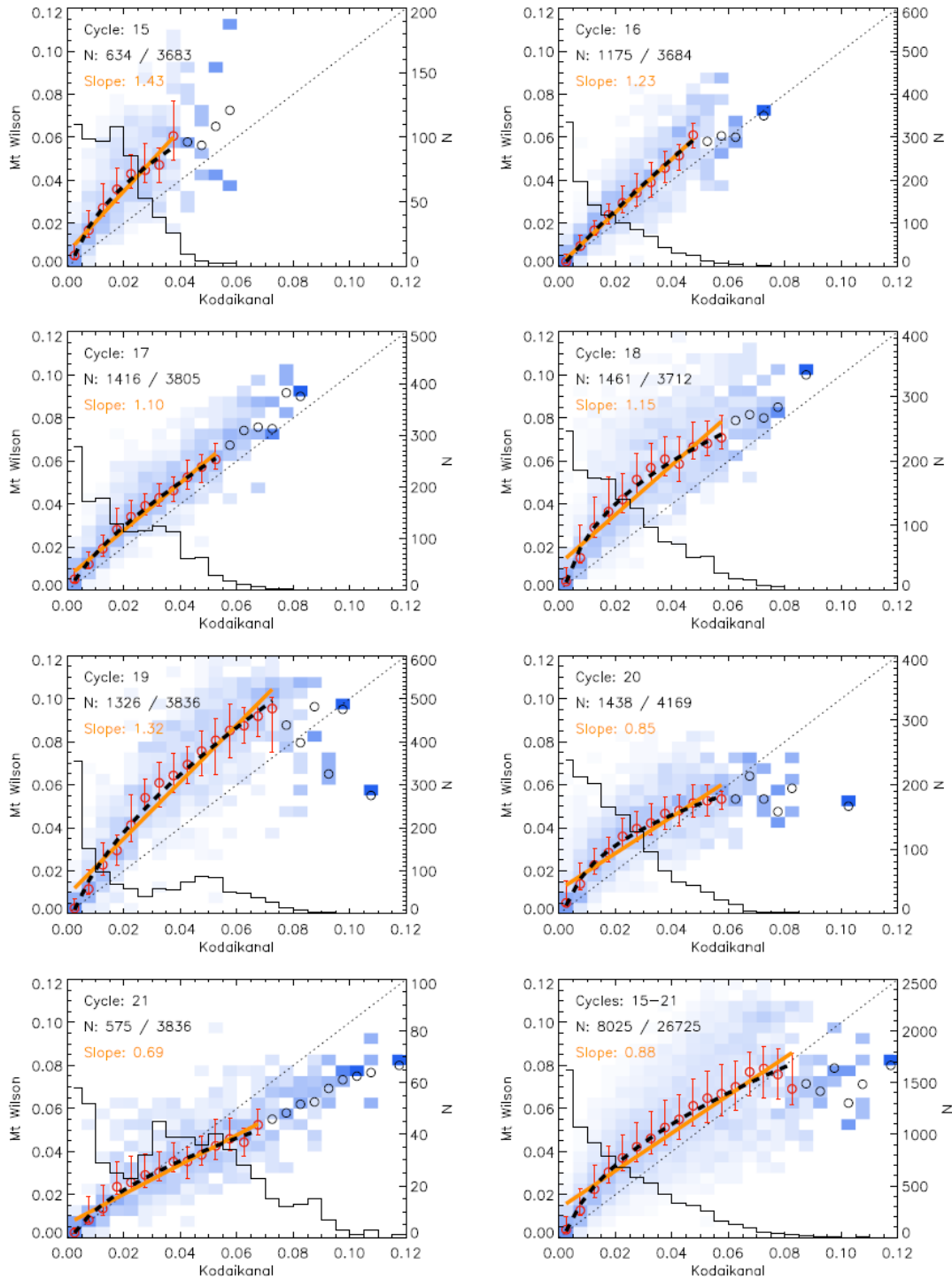
Fig. 8. Same as Fig. 7 but using MW plate area series as the reference and Ko as the secondary set.
