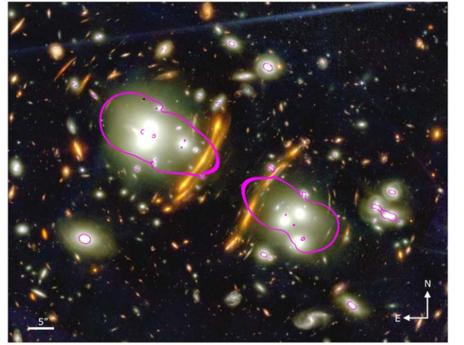
Figure 12. Color image using all NIRCam filters showing the central region of the G165 cluster. Magenta curves depict the z = 2 tangential critical curve obtained from our LTM model, and white labels show the image scale and orientation. Several giant arcs merge with the critical curve, an attribute that may assist with the detection of transients. The lens model separates out the northeastern and southwestern cluster cores at this redshift. The color rendering is the same as Figure 3.
