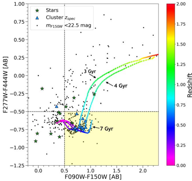
Figure 11. NIRCam color-color plot bracketing the rest-frame 1.6\ \mu\text{m} bump used to select G165 members at z = 0.35 . Small points show galaxy colors measured by NIRCam. Blue triangles indicate cluster members selected by spectroscopic redshifts, and green stars indicate Milky Way stars. The yellow-filled region in the lower right shows the color-selection area for cluster members. The colored lines show colors of stellar populations of 3, 4, and 7 Gyr at 0.1 < z < 1.5 with redshift encoded as shown by the color bar. These colors represent a low-dust elliptical galaxy with no active galactic nucleus (AGN).
