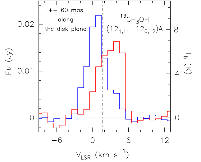
Fig. A.3: Comparison in flux density and in T_B scales ( T_B/F_\nu = 482.609 \text{ K Jy}^{-1} ) between the ^{13}\text{CH}_3\text{OH(12}_{1,11}\text{--12}_{0,12}\text{)A} spectrum extracted at \pm 0.06 from the protostar (see Fig. 2: blue- and red-shifted emission towards North-West and South-East, respectively) in the direction along the equatorial plane (i.e. disk plane; Lee et al. 2017). The vertical dashed line stands for the systemic V_{\text{LSR}} velocity (+1.7 km s ^{-1} , Lee et al. 2014).
