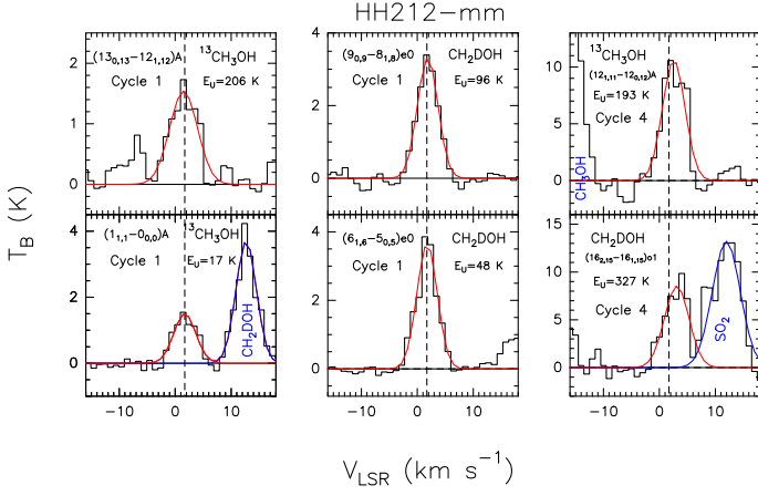
Fig. A.1: Examples of line profiles in T_B scale (not corrected for the beam dilution): species and transitions are reported. The vertical dashed line stands for the systemic V_{LSR} velocity (+ 1.7 km s -1 , Lee et al. 2014). Red and blue curves are for the Gaussian fit. In the spectrum of Cycle 1 (1 1,1 -0 0,0 )A 13 CH 3 OH transition, a CH 2 DOH doublet containing the (5 4,2 -5 3,2 )e1 and the (5 4,1 -5 3,3 )e1 transitions is also shown (see Table A.1). In Cycle 4 spectra the (7 1,7 -6 1,6 )A CH 3 OH and the (8 2,6 -7 1,7 ) SO 2 transitions are also shown.
