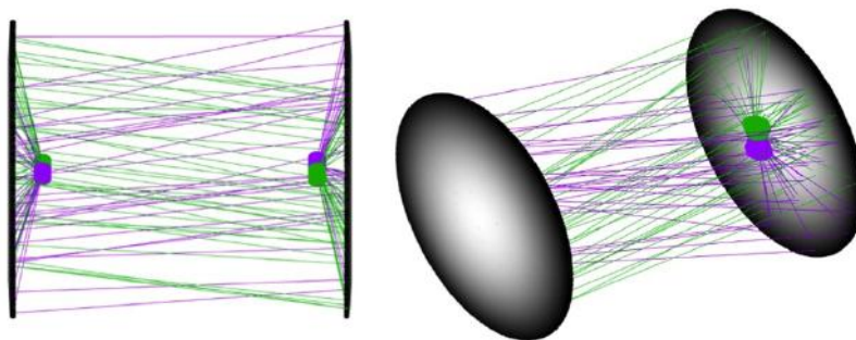
Figure 8. Ray tracing of the two parabolas system for a source as the one used in the experiment. The image is inverted.
