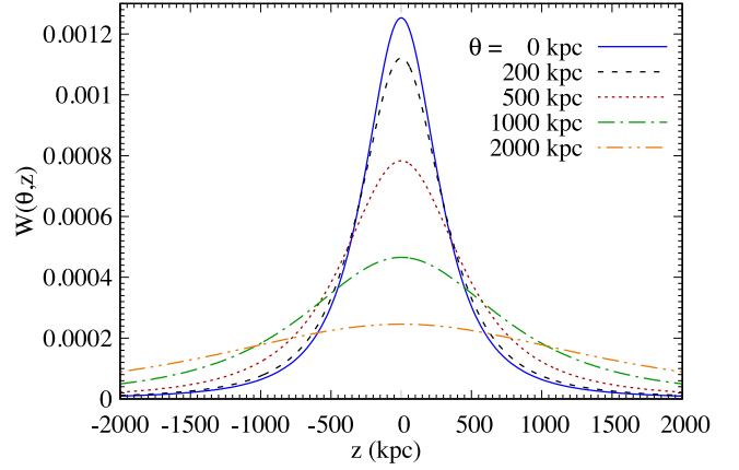
Figure 7. The window function W(\theta, z) at several values of the projected distance \theta from the centre. As we get away from the centre, the window profile becomes broader increasing the suppression of the small-scale power.
