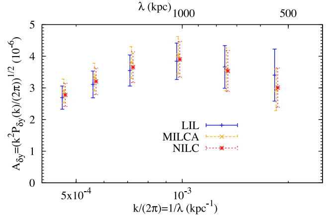
Figure 5. Power spectrum of fluctuations of y , \delta y = y - \bar{y} , in Coma with the average profile subtracted for MILCA, NILC and LIL maps. The NILC data point is at the centre of the k bin, while the other data points are slightly offset to make them distinguishable from each other.
