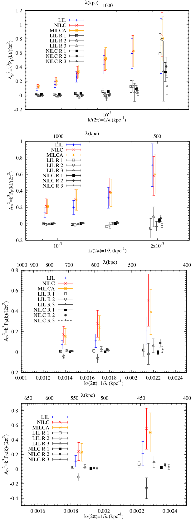
Figure 12. Squared amplitude spectrum of Coma pressure fluctuations for \theta_{\text{max}} = 60, 30, 20, 15 arcmin (top to bottom) in LIL, MILCA and NILC maps and in the test regions (LIL maps). For the test region we used our best-fitting Coma profile in the denominator to calculate \delta y/\bar{y} .
