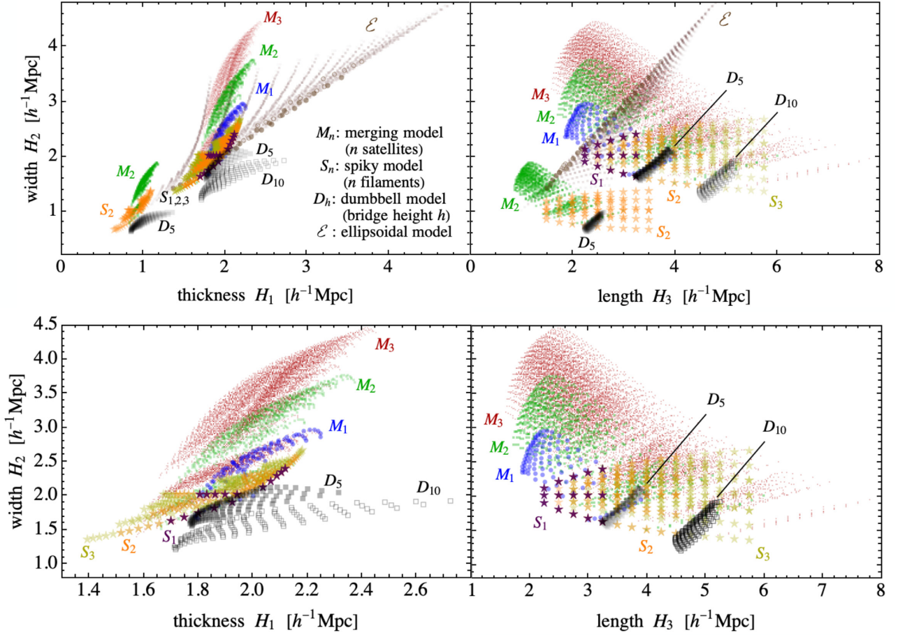
Figure 6. Classification by shapefinders ( H_1, H_2, H_3 ) of ellipsoidal triaxial, merging, spiky, and dumbbell models in two projections (left- and right-hand panels; see Section 3 for values). Top panels: merging, spiky, and dumbbell models have central or major ball with radius R = 1 or 2h^{-1} Mpc. Correspondingly, they have H_1 \approx 1 or 2h^{-1} Mpc and H_2 \gtrsim 1 or 2h^{-1} Mpc. Bottom panels: zoom on models with major ball with R = 2h^{-1} Mpc.
