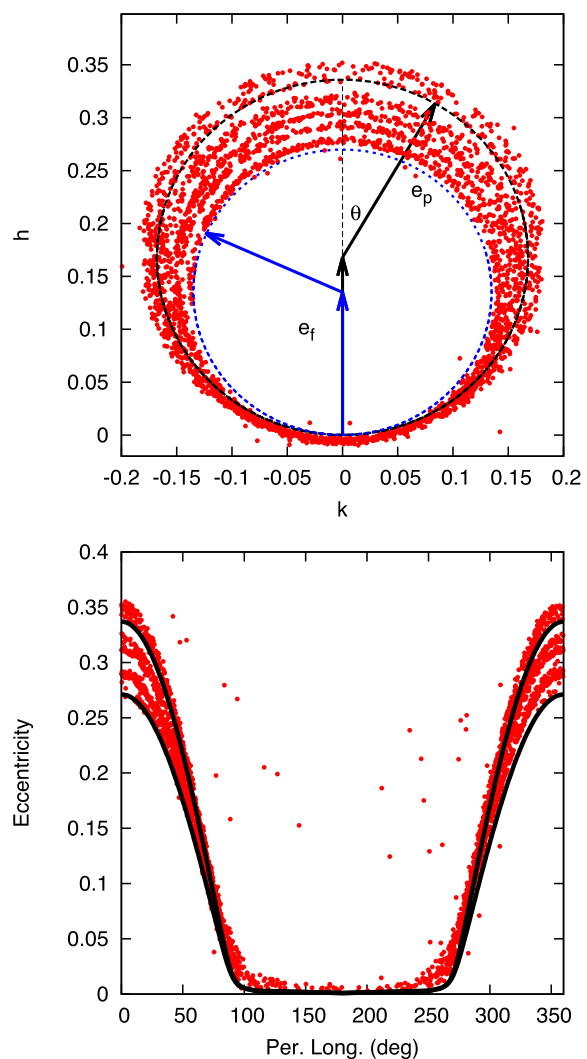
Figure 1. Secular evolution of a population of planetesimals moving in a ring with semimajor axis ranging from 15 to 20 au and initially circular orbits. They are perturbed by a Jupiter-sized planet with a_{pl} = 5 au and eccentricity e_{pl} = 0.5 . In the top panel, the evolution of the non-singular h and k variables is illustrated [ h = e \cos(\varpi) , k = e \sin(\varpi) ]. The arrows show the forced e_f and proper e_p eccentricities for a = 15 au (in blue) and a = 20 au (in black), which, once combined, give the eccentricity of the planetesimals. The blue and black dashed lines show the curves obtained by combining proper and forced eccentricity. In the bottom panel, the correlation between \varpi and e is highlighted.
