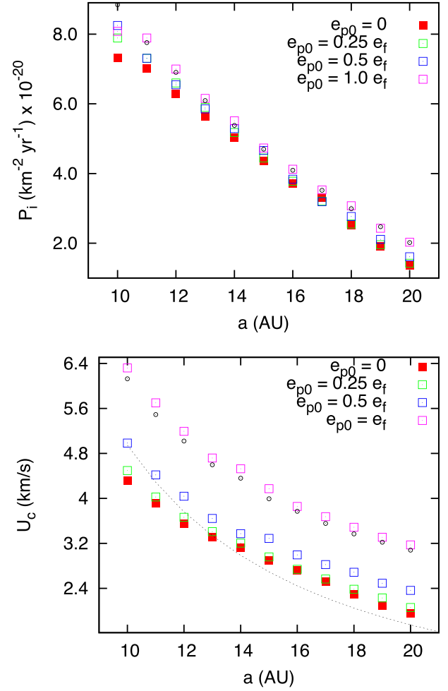
Figure 8. Same as Fig. 7 but for e_{pl} = 0.6 .
