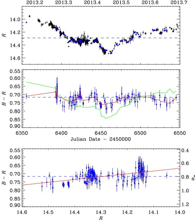
Figure 3. Top: the R -band light curve (black plus signs) where data points used to build the B - R colour indices have been highlighted with blue dots. Middle: B - R versus time; the red line represents the smoothed trend of the colour index; the green line the smoothed R -band light curve ( R/2 - 6.4 ). Bottom: B - R and optical spectral index \alpha_o versus brightness; the red line represents a linear fit to the data. Horizontal dashed lines mark mean values.
