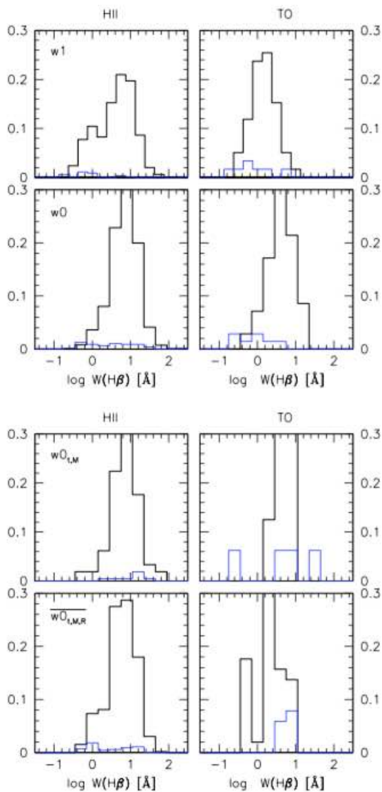
Fig. 6. Distribution of W(H\beta) (in Å) for sources classified as HII (left), and TO (right), for w1, w0, one realization of w0_{t,M} and w0_{t,M,R} (from top to bottom). The black histograms trace the distribution of detections, the thin blue ones the distributions of upper limits.
