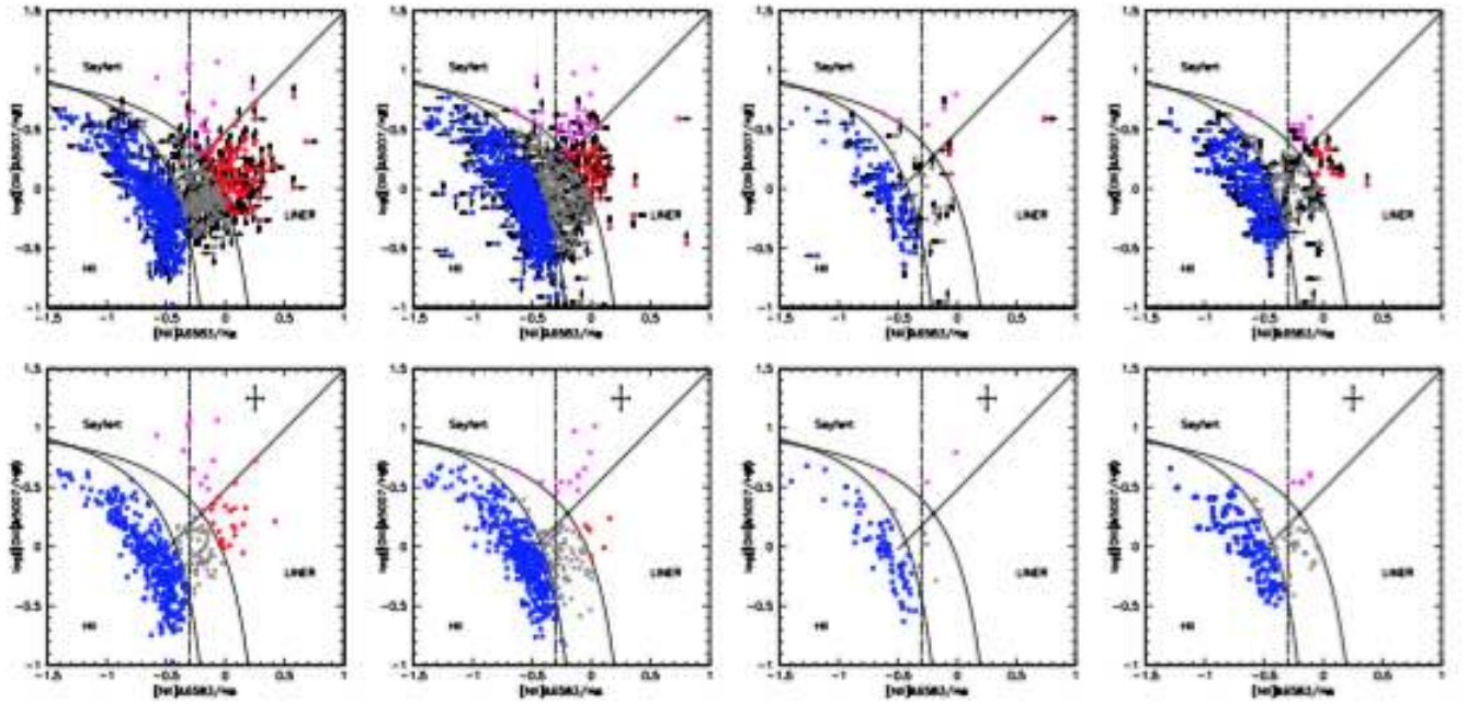
Fig. 7. [\text{OIII}]\lambda 5007/\text{H}\beta vs [\text{NII}]\lambda 6583/\text{H}\alpha diagnostic diagrams. Leftmost panel: DD for galaxies that are cluster members; second panel from right: same, for w_0 . The third and fourth panels from right show one realization of w_{0,t,M} and of \overline{w}_{0,t,M,R} . Blue, red and magenta colors identify HII, LINERs and Seyferts respectively. Grey data points identify transition objects. Arrows indicate data points for which upper and/or lower limits to the diagnostic emission line ratios are considered. The bottom rows shows panel for detections ordered in the same sequence. Median errors at a 1\sigma confidence level are shown in the upper right corner of the diagrams with detections only.
