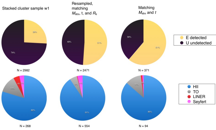
Fig. 3. Top: fractions of quiescent galaxies (black), and ELGs (yellow), for w1 cluster galaxies (left), one realization of w0 t,M,R and w0 t,M (middle and right). Bottom: prevalence of different ELG classes identified in the DD [NII] from uncensored diagnostic ratios: HII (blue), transition objects (pale grey), LINERs (red) and Seyferts (magenta), ordered as in the top row.
