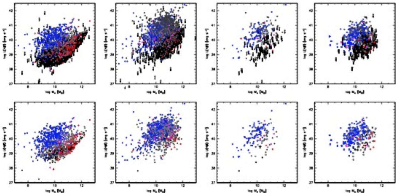
Fig. 12. Logarithm of H \beta luminosity in erg s ^{-1} versus log of stellar mass in solar units, for cluster members and non-members (middle and right panels), in the following order from left to right: w1, w0, one realization of w0 _{t,M} , one realization of w0 _{t,M,R} . Upper panels include upper limits and detections, lower panels are for detections only. Sources of different classes are identified by the same color coding of the previous Figures.
