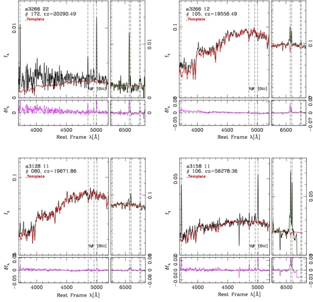
Fig. 2. Examples of ELG spectra. Top left: the high-ionization HII galaxy WINGS J043319.43-614141.8; the TO WINGS J043021.56-612848.7; bottom left: the LINER WINGS J032933.77-522659.6; bottom right the Seyfert 2 galaxy WINGS J034144.52-534221.1. Red lines trace the adopted stellar template. All of these sources could be entered in the DD with detected diagnostic ratios, and have probability of proper classification P_{i,i} \gtrsim 0.8 .
