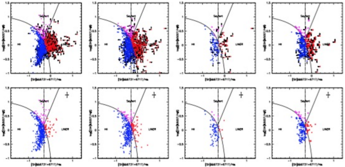
Fig. 10. [\text{OIII}]\lambda 5007/\text{H}\beta vs [\text{SII}]\lambda\lambda 6716,6731/\text{H}\alpha diagnostic diagrams. Meaning of panel and symbols and disposition of panels is the same of Fig. 7
