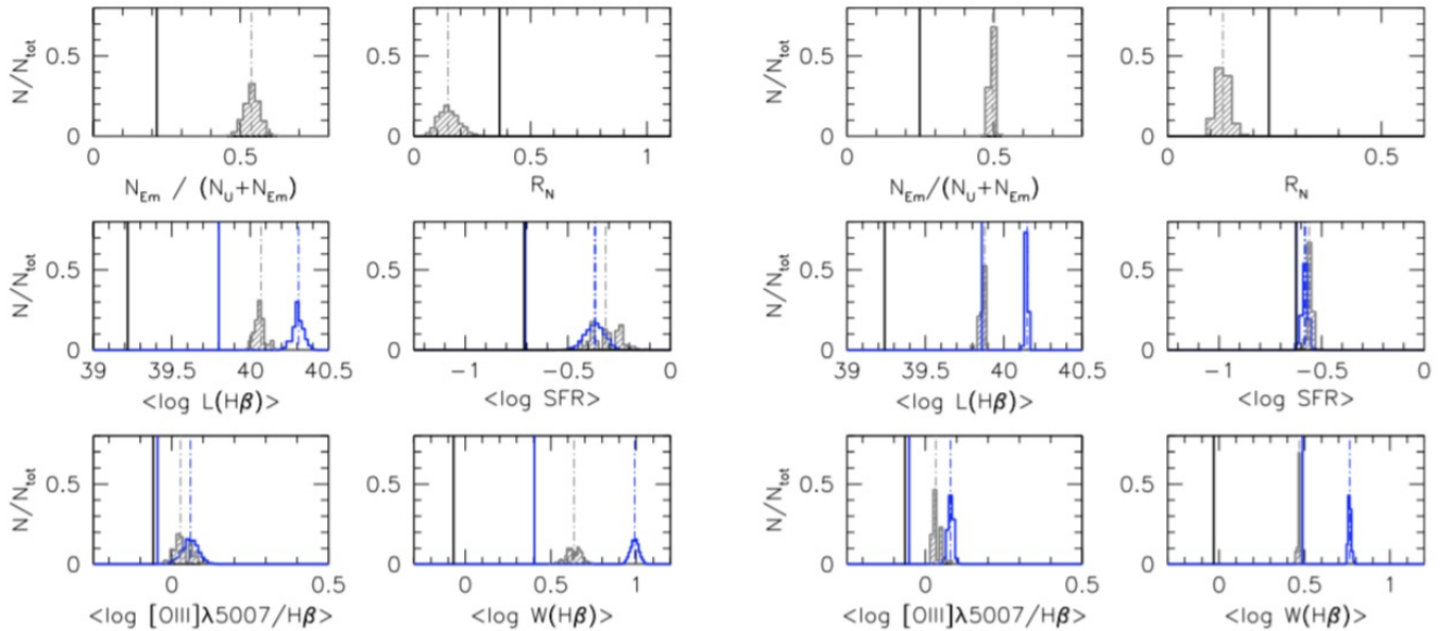
Fig. 5. Results of bootstrap simulations. The w1 sample is compared with 1000 virtual w0_{t,M} CSs of \approx 350 sources (six leftmost panels), and with 200 virtual w0_{t,M,R} (six rightmost panels). The panels show median values measured for the cluster members (thick solid lines) along with the distributions of the bootstrapped sample w0_{t,M} medians (left) and w0_{t,M,R} (right) and their medians (dot-dashed lines). Top: ratio R_{Em} (left), ratio R_N (from DD_{[NII]} ; right), for the revised classification (grey). The middle panels show the luminosity of H\beta in \text{erg s}^{-1} (left), and the SFR in M_{\odot} \text{ yr}^{-1} (only for HII sources; right). Blue histograms and lines refer to average values of detections only, grey histogram and lines show medians and include upper limits. Bottom panel: distributions for [OIII]\lambda 5007/H\beta (left) and W(H\beta) (right), with the same meaning of color coding.
