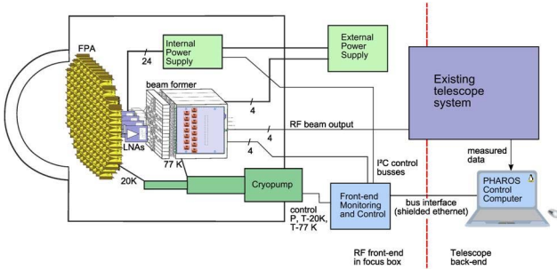
Figure 1. PHAROS system diagram.
