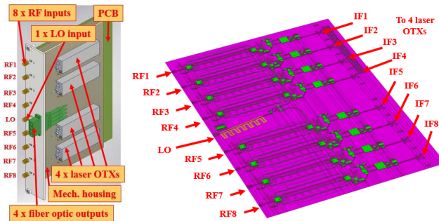
Figure 5. Left: Design of one of the WS RF/IF modules, which incorporates a PCB and four WDM fiber optics transmitters. Right: view of PCB layers and of RF/LO/IF components. The size of the PCB is 160 mm×233.4 mm.
