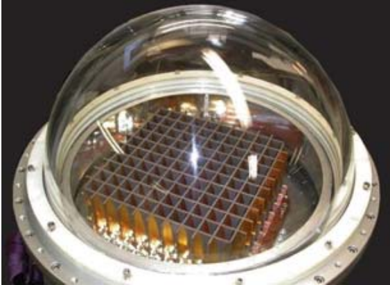
Figure 2. PHAROS focal plane array and dome-shaped vacuum window attached to the cryostat.
