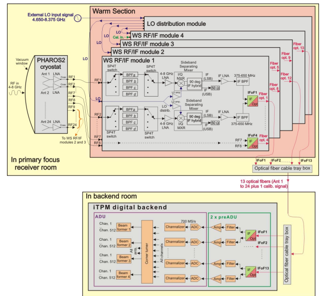
Figure 3. Schematic diagram of PHAROS2.
