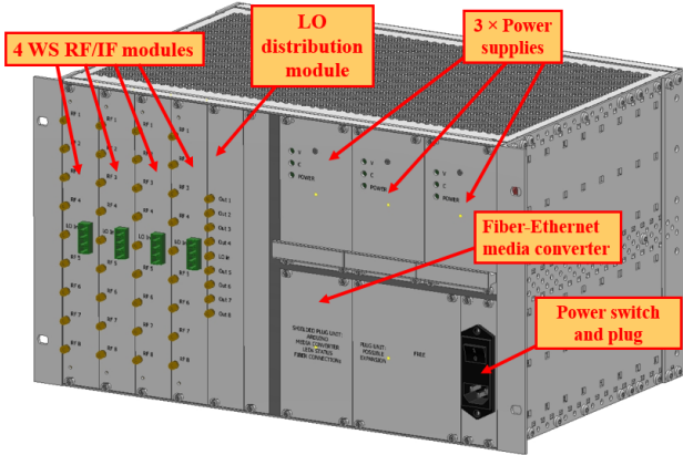
Figure 4. Design of PHAROS2 Warm Section.
