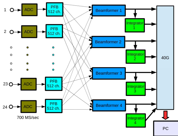
Figure 6. Implementation of PHAROS2 digital backend with beamforming performed in the iTPM-FPGAs.
