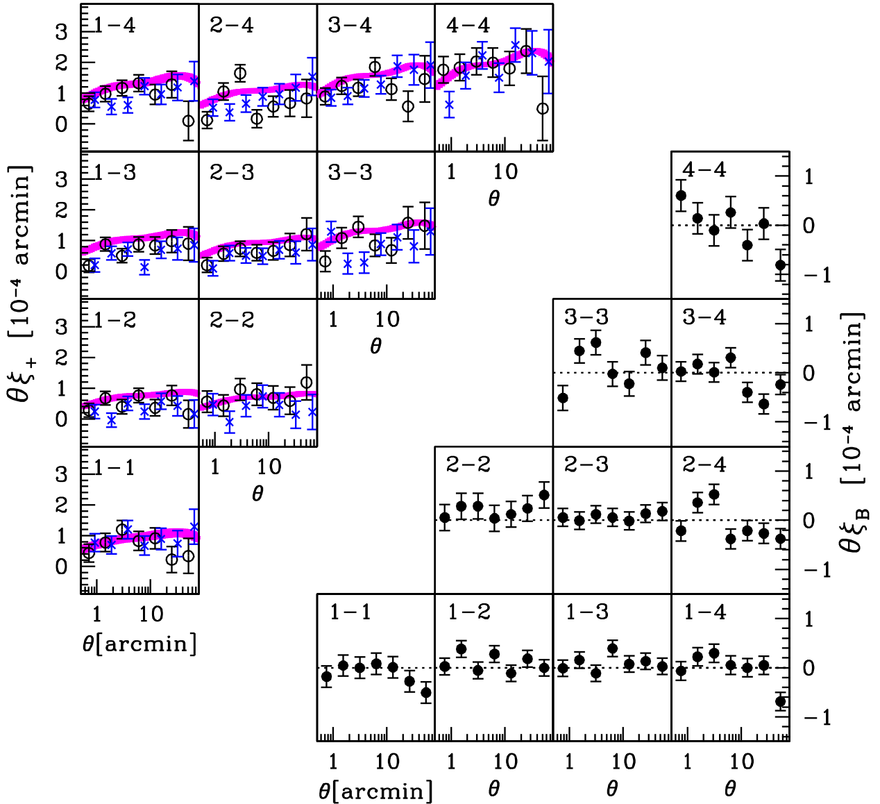
Figure D11. Tomography measurements using \xi_B for each redshift bin combination, as denoted in the caption inset in each panel. Lower right-hand panel: the measured B mode \xi_B (equation D7). Upper left-hand panel: Measurements of \xi_+^{\text{obs}} (open symbols) are corrected using the measured B mode (crosses, equation D11). The data with and without B-mode correction can be compared with the best-fitting cosmological model (solid) with its own error arising from uncertainty in the measured DIR redshift distribution.
