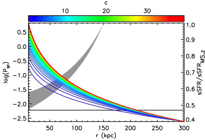
Fig. 11. Decrease in sSFR in a simple no-infall, no-recycling case as a function of distance to the center of the halo (gray, right axis; arbitrarily starting at r = 150 kpc) and tidal perturbation parameter P_{gc} (red to blue, left axis), for a low-mass satellite. The horizontal line shows the threshold value at which the gravitational influence of the halo can trigger inflow within satellite galaxies (Byrd & Valtonen 1990). Both quantities are shown for NFW concentration parameters ranging from c = 1 to c = 40 .
