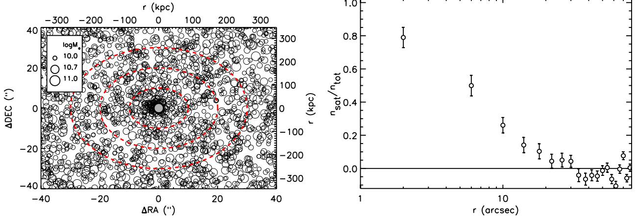
Fig. 3. Left: positions of all satellite candidates (open circles) compared to their respective centrals (filled circle), with the overdensity most visible at \leq 10'' . The size of each symbol varies as a function of its stellar mass. The red dashed contours show scales of 10'' , 20'' , and 30'' , respectively. Right: fraction of expected “real associations” among satellite candidates, n_{\text{sat}}/n_{\text{tot}} as a function of radius (where n_{\text{sat}}(r) = n(r) - n_b , n(r) and n_b being, respectively, the number density of satellite candidates at radius r and at >50'' ).
