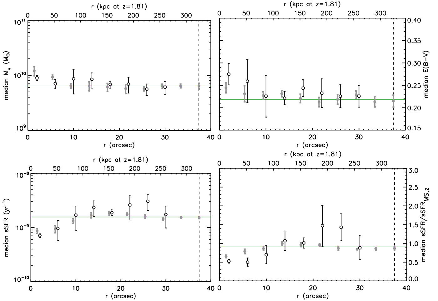
Fig. 9. Median background-subtracted stellar population parameters of UVJ -selected star-forming satellites (open symbols), as a function of distance to the central, in bins of 4'' : stellar mass ( top left ), extinction ( top right ), sSFR ( bottom left ), and sSFR as a fraction of the main-sequence value (assuming a slope of 0.8). Median values for the total distribution of star-forming satellites (i.e., without subtracting the background distribution) are shown in gray, slightly shifted to the left for convenience. Background levels and related uncertainties, estimated at r > 50'' , are shown in green and the virial radius is indicated by a dashed line.
