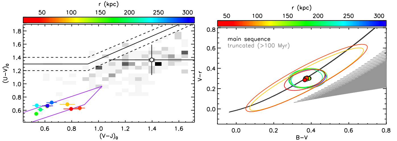
Fig. 10. Left: median rest-frame U - V and V - J colors, derived from SED modeling, of star-forming satellites (filled circles, colored as a function of distance to the central) and centrals (open circle and gray density histogram). The purple lines show the expected colors of stellar populations models of varying age following a “main-sequence” SFH, assuming E(B - V) < 0.3 . Right: median observed B - V and V - r colors of satellites, as a function of distance to the central, compared to the expected colors of a star-forming model (main-sequence SFH, black) and a constant SFR one observed \geq 100 Myr after the quenching of star formation (gray). We here include dust extinction with E(B - V) = 0 - 2 . The ellipses show the dispersion of B - V and V - r values in each radial bin.
