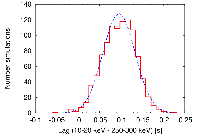
Figure 11. Distribution of the spectral lag analysis.
