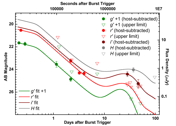
Figure 2. Light curves of the afterglow and SN component of GRB 200826A in the g' , r' , i' , and H bands, after subtraction of the host galaxy contribution. The data have been modeled with a smoothly broken power law for the afterglow, and with an SN 1998bw template redshifted to z = 0.7486 for the SN phase. In the g' and r' bands, we forced the individual SN light-curve components to go through the most significant deep upper limit in each band to obtain upper limits on the potential SN luminosity. Note the g' band is offset by 1 mag for reasons of clarity. See Table 1 and Sections 2.4 and 3.3 for more information.
