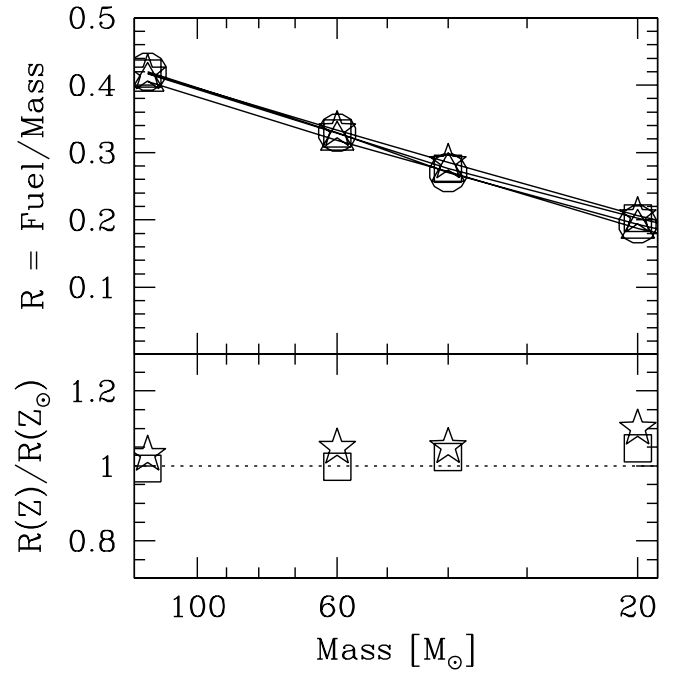
FIG. 5.— Top panel : Fraction of (initial) stellar mass consumed during MS evolution according to the Padova (Bressan et al. 1993; Fagotto et al. 1994) and Geneva (Schaller et al. 1992) evolutionary tracks. The plotted quantity is R = \text{fuel}/\text{mass} where \text{fuel} = (L_{ZAMS}t_{MS})/(0.007c^2) converted to hydrogen-equivalent solar masses. Padova tracks are for Z_{\odot} (open triangles) and Z = 0.004 (stars), while Geneva tracks are for Z_{\odot} (open circles) and Z = 0.001 (open squares). Bottom panel : Relative change in MS fuel consumption for the Padova Z = 0.004 tracks with respect to the solar case (stars) and, similarly, for the Geneva Z = 0.001 tracks (open squares).
