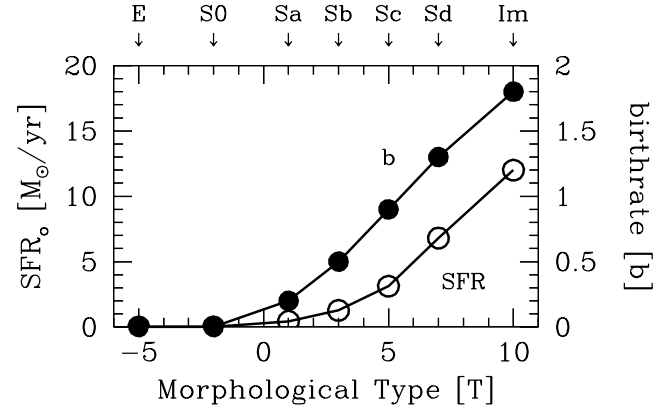
FIG. 8.—Current SFR for disk stellar populations as expected from our template models for different morphological types (left scale refers to open circles in the plot). A total mass of 10^{11} M_{\odot} is assumed for the galaxies. Right scale reports the mean birthrate b = \text{SFR}_0 / \langle \text{SFR} \rangle according to Table 3 ( filled circles ).
