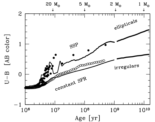
FIG. 10.—Theoretical U-B colors (in AB magnitude scale) for primeval galaxies with continuous star formation (“bluer” models) and SSP evolution (“redder” models). Models with Z_{\odot} and Salpeter IMF from Leitherer & Heckman (1995) (open and filled circles) and Leitherer et al. (1999) (thin solid lines) are compared with our reference templates for E and Im galaxies (thick solid lines; for t \geq 1 \text{ Gyr} ). The SSP evolution consistently matches early-type systems at later epochs, while a constant SFR suitably describes late-type and irregular galaxies. The SSP TO stellar mass at different epochs is reported on the top scale, according to eq. (3).
