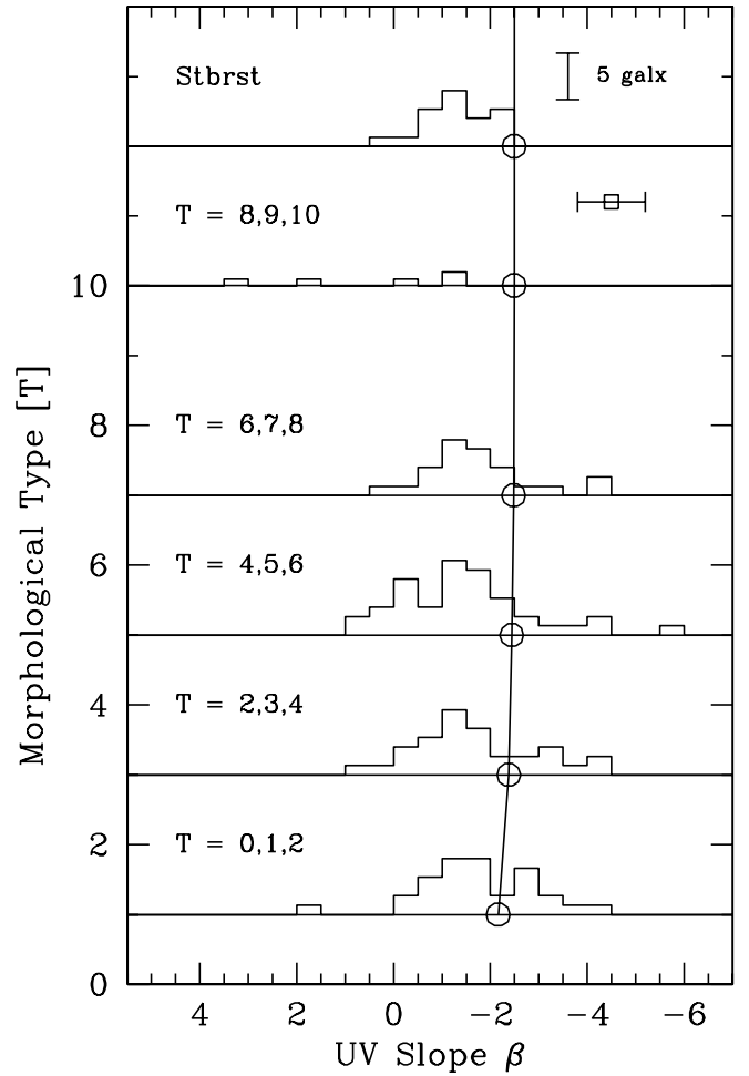
FIG. 14.—Observed distribution of the UV spectral slope, \beta = \Delta \log L(\lambda) / \Delta \log \lambda , for 19 starburst galaxies from Gordon et al. (1997) (top panel) and 93 spirals and irregulars ( T \geq 0 ) from the IUE catalog of Rifatto et al. (1995). The latter sample has been grouped in five bins according to the morphological parameter T , as labeled in the different panels. Only the Gordon et al. data have been originally corrected for Galaxy reddening. Open circles and the solid line mark the theoretical lower limit to \beta according to our 15 Gyr template models (i.e., \beta = -2.4 ). The reddening vector is \Delta\beta/E(B - V) = 3.1 according to Seaton (1979), while internal attenuation is \Delta\beta/E(B - V) = 4.5 following Calzetti (1999). The typical uncertainty in the observed UV slope is \sigma(\beta) \sim \pm 0.7 for Rifatto et al. (as displayed top right in the plot) and \sigma(\beta) \sim \pm 0.25 for the Gordon et al. galaxies.
