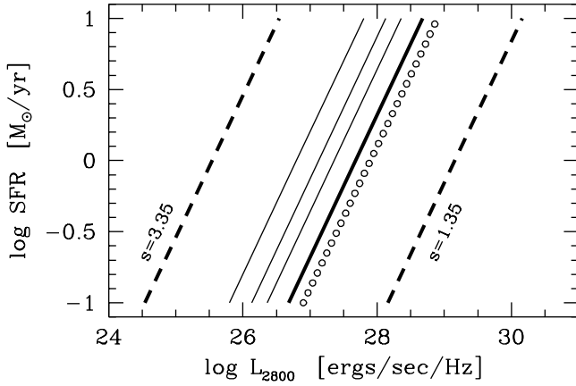
FIG. 4.—Theoretical L_{UV} vs. SFR calibration at 2800 Å according to eq. (6). Solid lines (left to right) refer to a Salpeter IMF ( s = 2.35 ) and M_{up} = 40, 60, 80 , and 120 M_{\odot} , with the last case marked in boldface. The IMF slopes for s = 3.35 and 1.35 and M_{up} = 120 M_{\odot} are shown by the two dashed lines. The Madau et al. (1998) calibration for a Salpeter IMF and M_{up} = 125 M_{\odot} is also given for comparison (dotted line).
