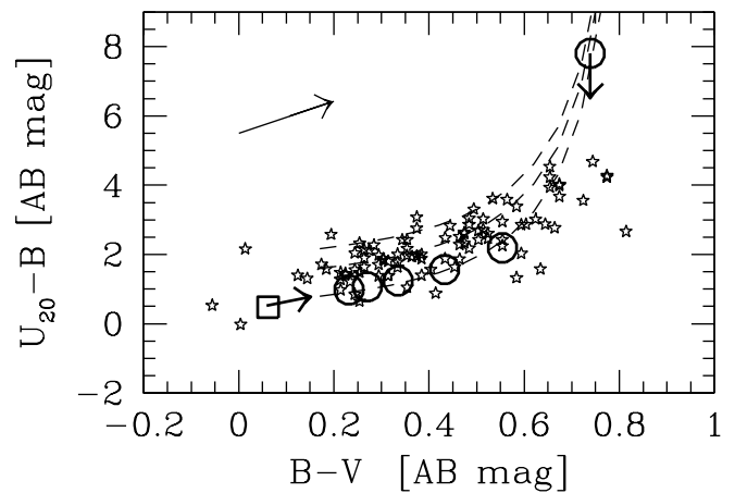
FIG. 13.—Two-color diagram of the 149 late-type galaxies in the Donas et al. (1987) sample (stars). Large open circles show the locus for 15 Gyr template galaxies along the sequence \text{Im} \rightarrow \text{E} , in the sense of increasing B - V . The Im model at 1 Gyr is also displayed (large open square). Reference models assume a Salpeter IMF with M_{\text{up}} = 120 M_{\odot} . The effect of residual star formation in the early-type templates is indicated by the vertical arrow on the E model. A change in the IMF upper cutoff mass for M_{\text{up}} to 80 and 60 M_{\odot} , in the sense of “reddening” U_{20} - B , is explored by the dashed curves. All the colors in the plot are in AB magnitude scale. Galaxy reddening is accounted for in the original observations. The reddening vector at the top left is from Seaton (1979). The typical error bar for the UV data is \pm 0.5 mag on U_{20} - B .
