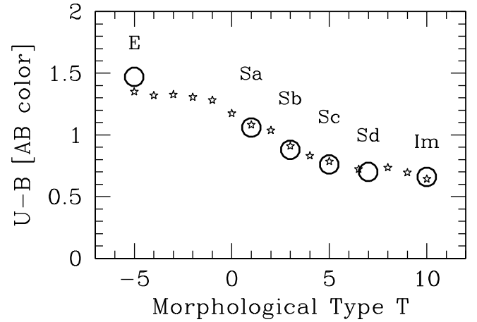
FIG. 9.—Mean observed locus for RC3 galaxies of different morphological type (stars) according to Buta et al. (1994), compared with 15 Gyr galaxy templates (large open circles). The Johnson U-B color is in AB magnitude scale. Data have been originally corrected for Galaxy and internal average reddening. The typical internal scatter of the observed points is \pm 0.1 \text{ mag} .
