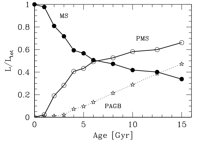
FIG. 2.—SSP luminosity evolution in the UV wavelength range ( \lambda < 3000 \text{ \AA} ) according to Buzzoni's (1989) synthesis code. A solar metallicity and a Salpeter IMF are assumed. The relative contribution from MS (filled circles) and post-MS (open circles) stars is compared. The luminosity fraction provided by post-AGB stars alone (stars) is also singled out.
