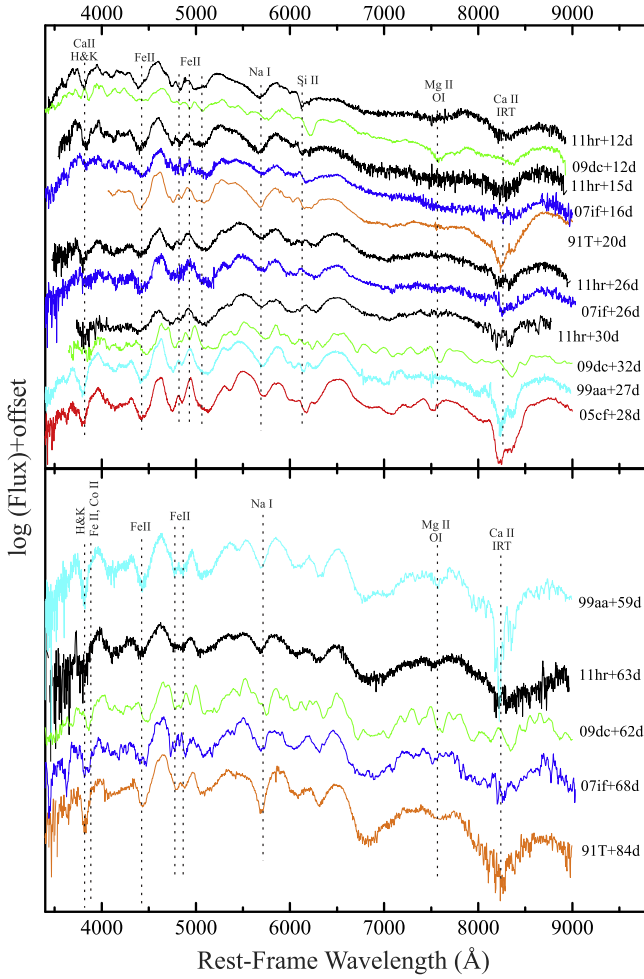
Figure 7. Postmaximum spectra of SN 2011hr, compared to the same SNe as in Figure 5. The spectrum of SN 2007if at t \approx +68 is smoothed with a box of 10 ( \sim 24 Å). The spectrum of SN 1999aa at t \approx +59 days is from Silverman et al. (2012).
