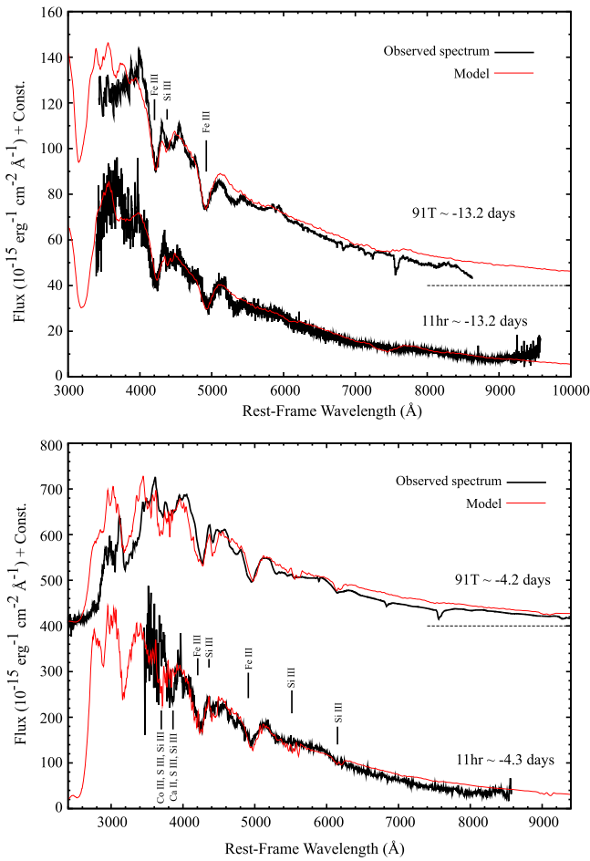
Figure 12. Synthetic spectra are compared with the observed spectra of SN 2011hr at -13.2 and -4.3 days. At the top of each panel, the model and the observed spectrum of SN 191T at the same epoch from Sasdelli et al. (2014) are shown for comparison. To allow the comparison between these two SNe, the flux of SN 2011hr has been scaled by putting it at the same distance as SN 191T. The spectra are in rest frame and corrected for reddening by the amount assumed during the modeling.
