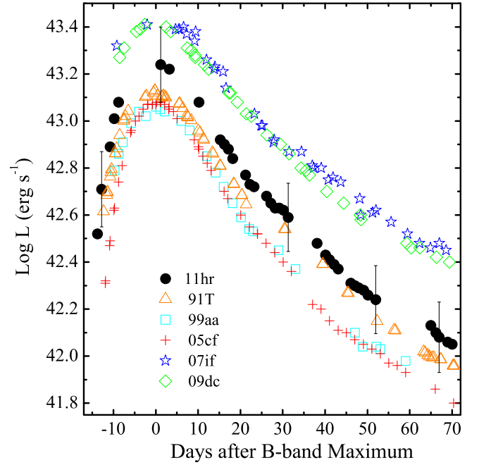
Figure 11. Quasi-bolometric light curves of SN 2011hr derived from the UBVR photometry, compared with those of SN 1991T, SN 1999aa, SN 2005cf, SN 2007if, and SN 2009dc.
