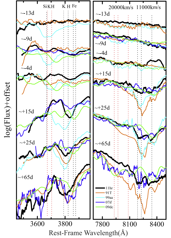
Figure 8. Evolution of the Ca II absorption in the spectra of SN 2011hr, SN 1991T, SN 1999aa, SN 2007if, and SN 2009dc at selected epochs. Left panel: evolution of Ca II H&K and Si II \lambda 3807 . Right panel: evolution of Ca II NIR triplet. The positions of Ca II H&K, Si II \lambda 3807 , Fe II, and the Ca II NIR triplet lines at different velocities (black dotted lines mark the line positions with v = 11,000 km s ^{-1} , and red dotted lines mark the positions with v = 20,000 km s ^{-1} ) are shown to guide the eyes. All spectra are smoothed with a boxcar of 10 (i.e., \sim 20 – 30 Å). See Figures 5, 6, and 7 for the exact phase of each spectrum.
