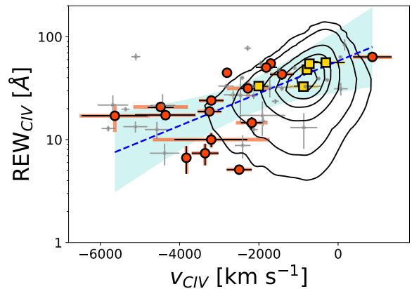
Fig. 3. The \text{REW}_{\text{CIV}} vs. v_{\text{CIV}} relation compared with the 0.05, 0.1, 0.3, 0.5, 0.68, 0.9 and 0.99 contour levels (relative to the peak) of the SDSS DR7 sample (Shen et al. 2011; Vietri et al. 2018) and with the values from Schindler et al. 2020 (grey points). For simplicity, we plot here the mean values derived using all the available values reported in Table 3. We note that the fit takes into account all the existing values of v_{\text{CIV}} and \text{REW}_{\text{CIV}} (see Section 3.2).
