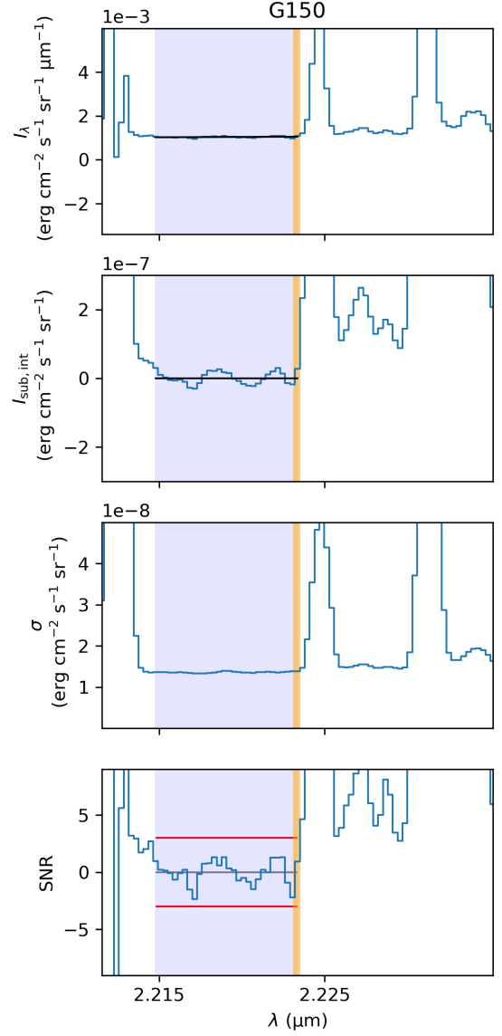
Fig. 2. Row 1: The 1D spectrum for G150 (see Appendix A for the rest of the targets). The black line is a linear fit to I_\lambda in the region with no skylines (blue strip). The vertical orange strip is the wavelength of the (1-0)\text{S}(0) line. Row 2: I_{\text{sub,int}} , the spectrum after we subtracted from it the linear fit and integrated over the instrument spectral resolution, \Delta\lambda \approx 7.4 \times 10^{-4} \mu\text{m} . Row 3: The error (noise) on I_{\text{sub,int}} . Row 4: the \text{SNR} = I_{\text{sub,int}}/\sigma . Wavelengths are in vacuum.
