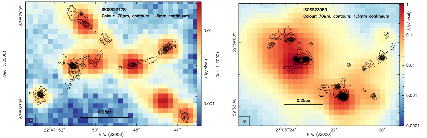
Fig. 2. NOEMA 1.3 mm continuum data for ISOSS22478 (left) and ISOSS23053 (right). The color scales show the 70 \mu m Herschel data and the contours present the 1.3 mm NOEMA continuum data. The contour levels are in steps of 3\sigma with the 1\sigma level of 57 \mu Jy beam -1 for ISOSS22478 and 160 \mu Jy beam -1 for ISOSS23053. Linear scale bars and the 1.3 mm beam size are shown.
