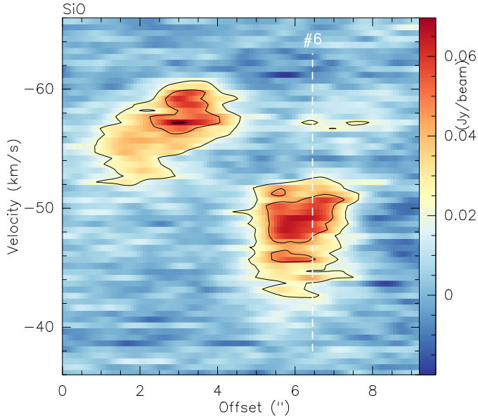
Fig. 14. Position-velocity diagrams in SiO(5–4) for source ISS23053 along the cut shown in Fig. 13 (middle panel). The contours are in 3\sigma steps of 22.5 \text{ mJy beam}^{-1} . The white dashed line marks the position of core #6.
