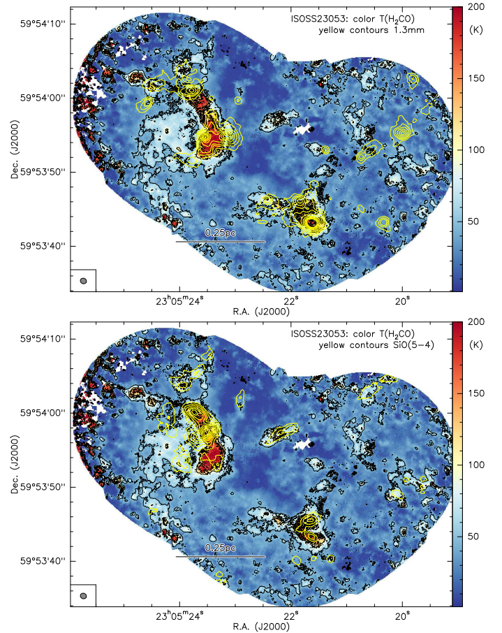
Fig. 15. Temperature map for ISS23053 derived from the \text{H}_2\text{CO} line emission. Both panels show, in color scale, the derived temperatures with black contour levels of 50, 100, and 150 K. The high temperatures in particular at the eastern edge of the map are not real but are caused by the lower signal-to-noise ratio there. The yellow contours in the top and bottom panels present the 1.3 mm continuum and the integrated SiO(5–4) emission, respectively. The 1.3 mm continuum contours are in 3\sigma steps ( 1\sigma \sim 0.16 \text{ mJy beam}^{-1} ). The SiO emission is integrated from -61 to -43 \text{ km s}^{-1} clipping all data below an approximate 4\sigma threshold of 20 \text{ mJy beam}^{-1} . Contour levels are from 10 to 90% (step 10%) of the integrated peak emission of 1.58 \text{ Jy beam}^{-1} \text{ km s}^{-1} . The beam is shown in the bottom-left of each panel, and a linear scale bar is shown as well.
