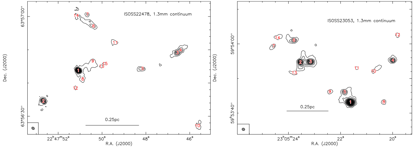
Fig. 3. NOEMA 1.3 mm continuum data for ISOSS22478 and ISOSS23053. The grey-scale and contours are now done in 5\sigma steps of 0.238 and 0.8 mJy beam -1 for ISOSS22478 and ISOSS23053, respectively. The red numbers label the identified cores. A linear scale bar and the 1.3 mm beam size are shown.
