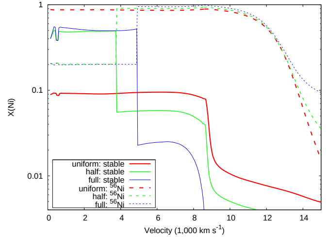
Fig. 3. Profile of ^{56}\text{Ni} and stable nickel in the inner regions of the ejecta of the models with M_{\text{WD}} = 1.06 M_{\odot} and Z = 0.035 with different distributions of ^{22}\text{Ne} (see Table 1 for details). The maximum velocity shown in the plot belongs to a Lagrangian mass coordinate \sim 0.91 M_{\odot} .
