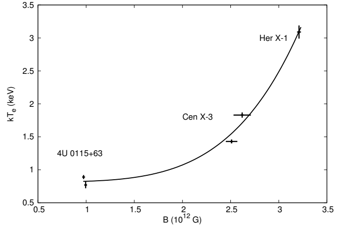
Fig. 5. Electron temperature as a function of the magnetic field at the base of the column for the sample of accreting X-ray pulsars analysed in this paper. The data values are given in Table 2 and can be fit by a power law (see text for more details).
