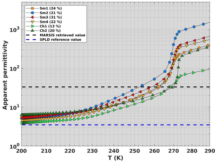
388 Fig.5 Apparent permittivity at 4 MHz from experimental data. Apparent permittivity computed from real and imaginary 389 parts measured at 4 MHz as a function of temperature on four smectite-rich (Sm) and two chlorite-rich (Ch) sediments 390 having different water content (% in the legend). Black dashed line indicates the threshold \epsilon_a = 33 retrieved by 391 MARSIS, and blue dashed line the SPLD ice permittivity value ( \epsilon_1' = 3.5 ) used to compute the apparent permittivity. 392 For clarity uncertainties are not shown in the diagram: they represent few percent of the measured values.
