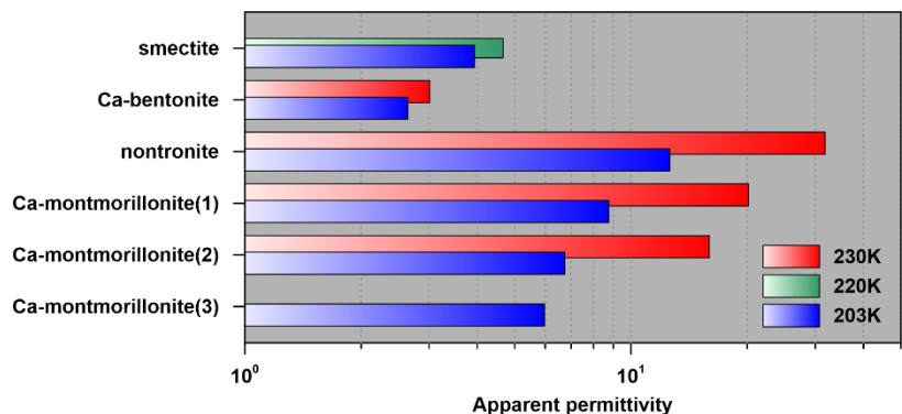
Fig. 3 Apparent permittivity at 1 MHz from literature data. Values of the apparent permittivity computed at 203 K and 230 K (220 K is from Stillman and Grimm (2011a), ref. to Table 2) from real and imaginary parts measured at 1 MHz on various smectite samples. The samples have different water content, clay content and salt solutions (Table 2).
