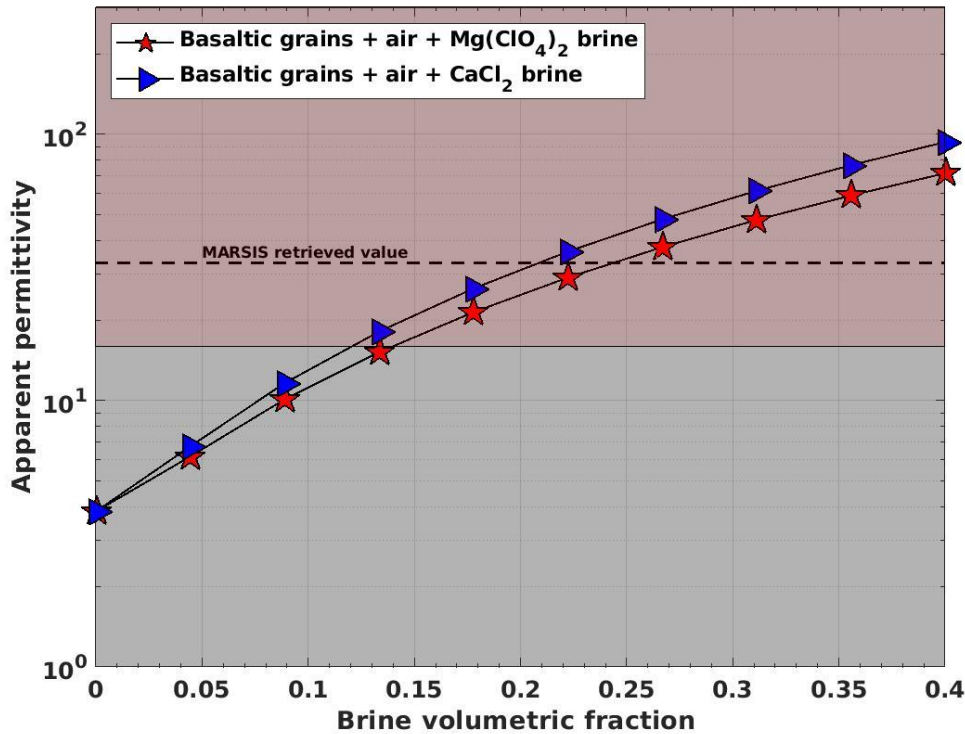
Fig.7 Effect of brines contents on the apparent permittivity of a soil from CRIM simulations at 4MHz. Apparent permittivity computed for a sandy soil with 40% porosity, from dry to brines saturated conditions. Blue triangles (33%wt CaCl 2 ) refer to the apparent permittivity measured at ~222K and red stars (44%wt Mg(ClO 4 ) 2 ) to the apparent permittivity measured at ~216K. Black dashed line indicates the threshold \epsilon_a = 33 retrieved by MARSIS; pink area highlights the apparent permittivity interval for which the probability that the permittivity assumes values \epsilon_a \geq 16 is 75%.
