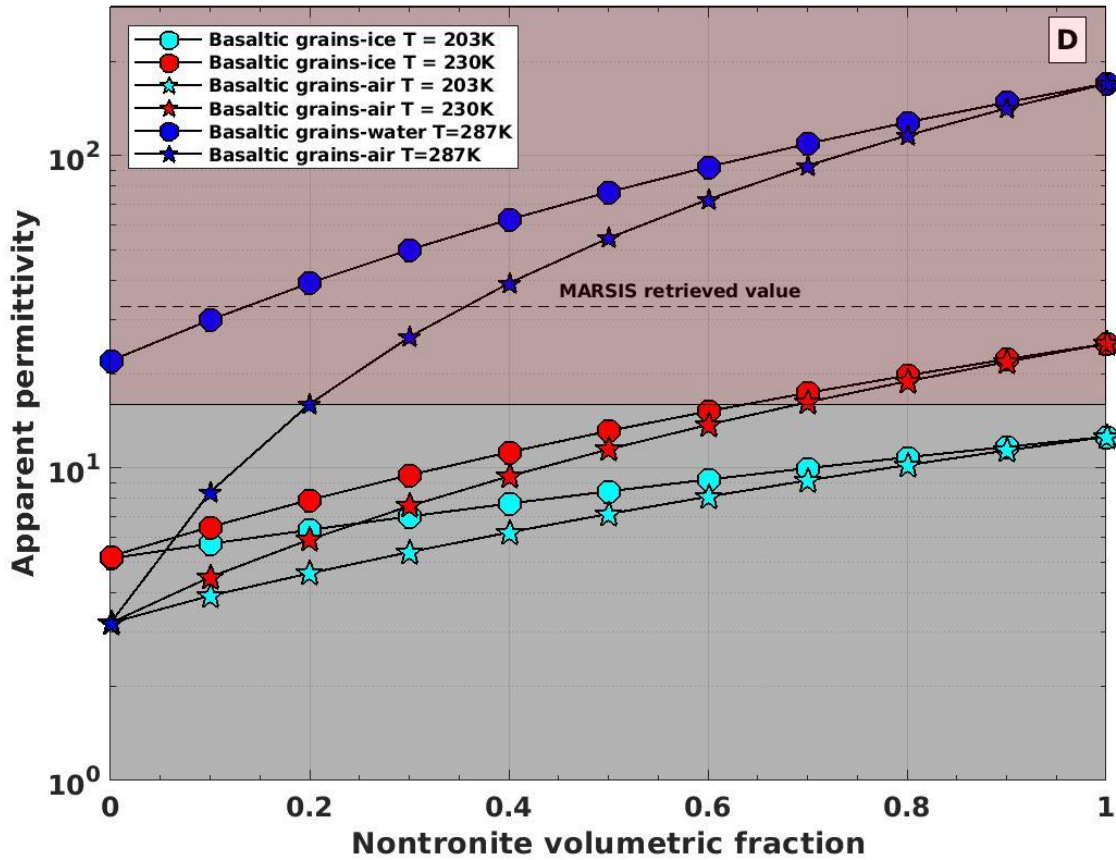
Fig. 4 Effect of nontronite content on the apparent permittivity from CRIM simulations at 4 MHz. A) desiccated Martian model; B) water ice saturated Martian model; C) terrestrial analogue. D) Different colors and shapes indicate different temperatures and mixtures: dots represent ice or water saturated mixtures; stars are dry samples (with air-filled pores). The ratio between the volume fraction of the basaltic grains and the material in the pore is held constant (1.5), with the nontronite volume fraction progressively increasing. The black dashed line indicates the MARSIS threshold value \epsilon_a = 33 ; pink area highlights the apparent permittivity interval for which the probability that the permittivity assumes values \epsilon_a \geq 16 is 75%.
