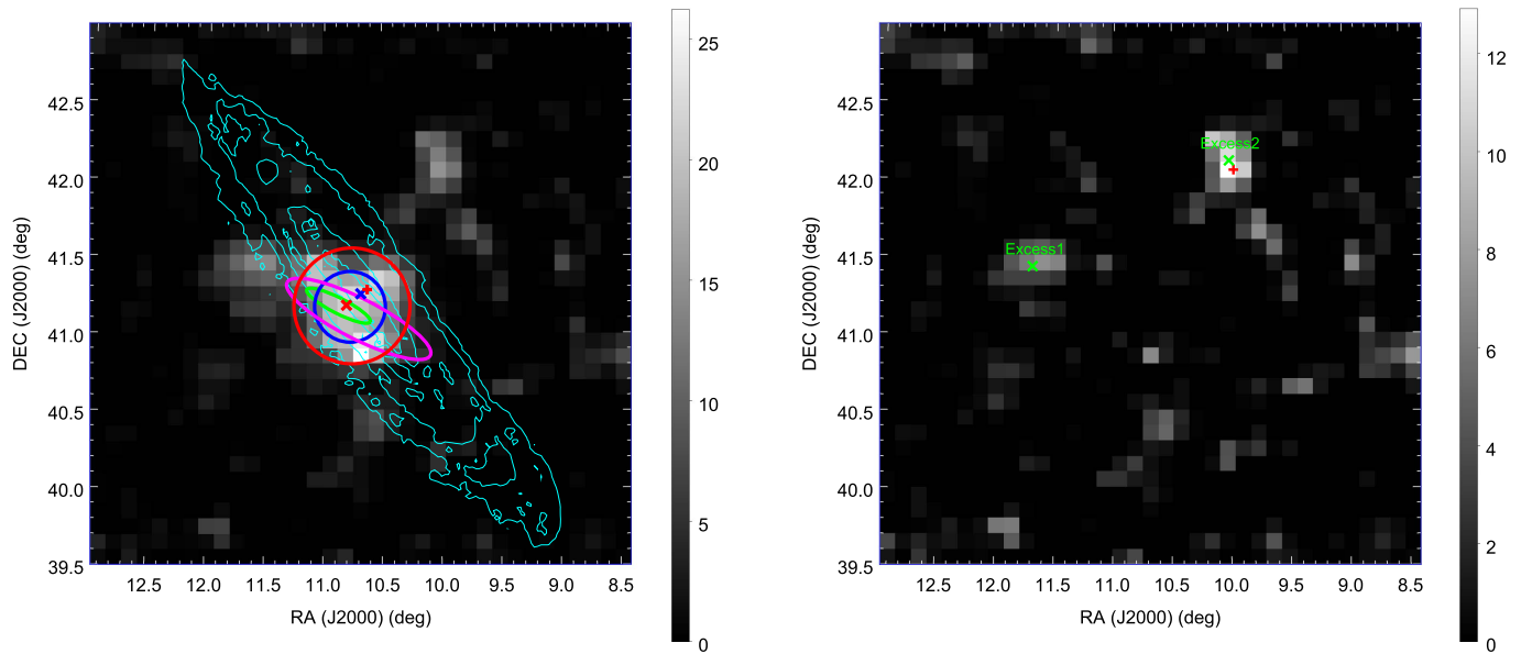
Figure 2. Left: TS map obtained for the background model, using 1–100 GeV events in a 3.5^\circ \times 3.5^\circ region around M31. Overlaid are the 3FGL position of M31 (the red plus sign), the center of M31 from SIMBAD (the blue cross), the best-fit point source position (the red cross), the best-fit disk (red circle), the best-fit elliptical disk (the magenta ellipse), the best-fit Gaussian (the blue circle, 1\sigma extent), the best-fit elliptical Gaussian (the green ellipse, 1\sigma extent), and contours of the atomic gas column density map (cyan curves). Right: TS map obtained for a source model including M31, using 1–100 GeV events in a 3.5^\circ \times 3.5^\circ region around M31. Overlaid are the positions of possible sources Excess1 and Excess2 (the green cross) and of the LAT 7 yr internal list source (the red plus sign). Both maps have a pixel size of 0.1^\circ .
