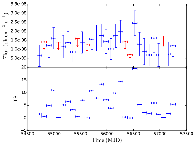
Figure 4. 0.1–100 GeV light curve and TS evolution for M31 (left) and the source in the direction of M33 (right), with 90-day binning. Flux ULs at the 95% confidence level are shown as red arrows in bins where the source has TS < 1 .
